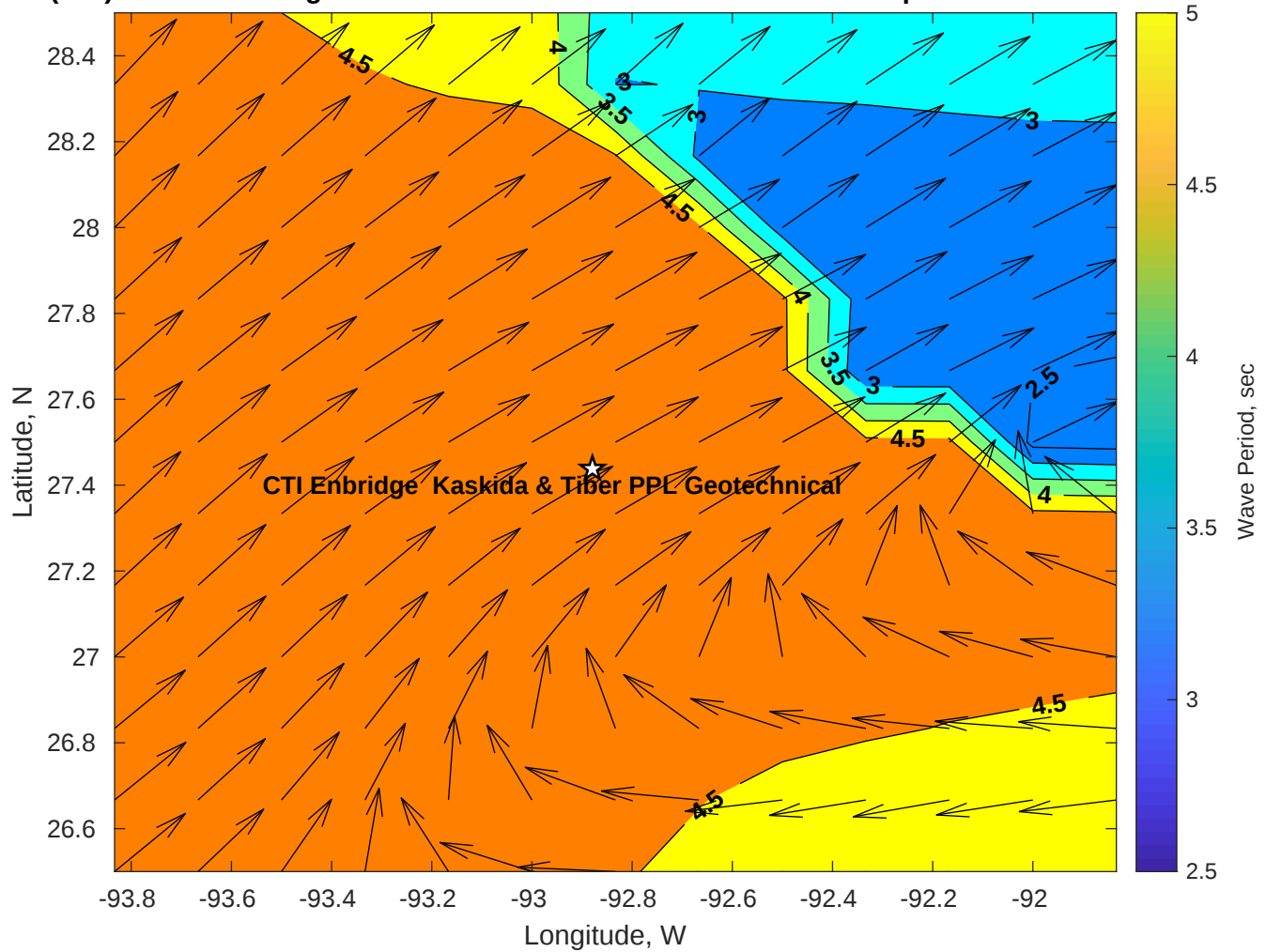
Wave Period (sec) for CTI Enbridge Kaskida & Tiber PPL Geotechnical at 11-Apr-2025 09:00:00
