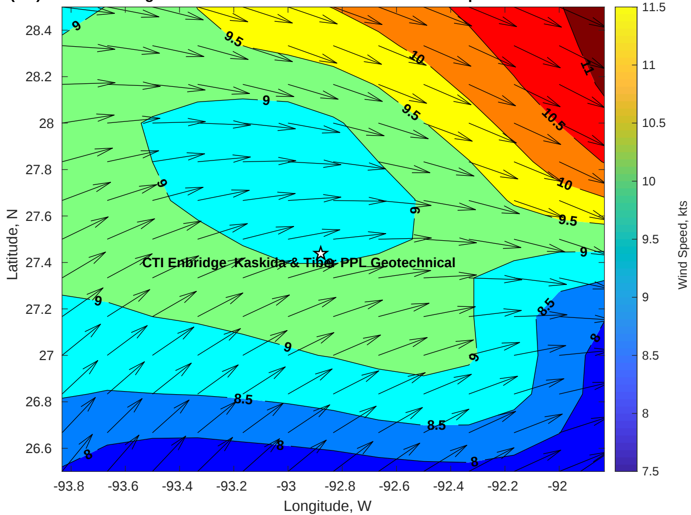
Winds (kts) for CTI Enbridge Kaskida & Tiber PPL Geotechnical at 11-Apr-2025 09:00:00
