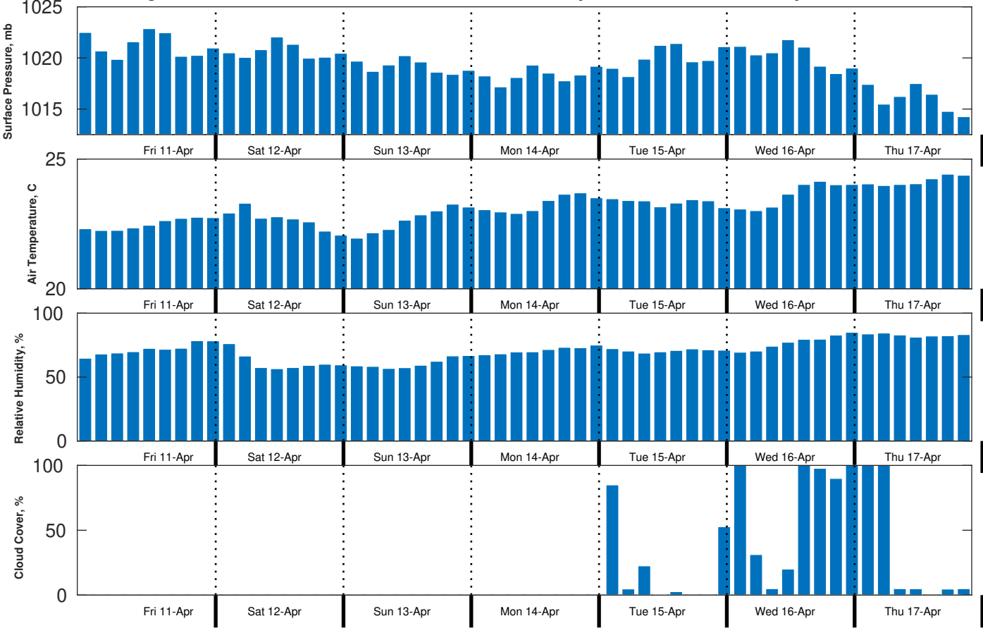
Met Forecast for CTI Enbridge Kaskida & Tiber PPL Geotechnical from 11-Apr-2025 00:00:00 to 18-Apr-2025 00:00:00
