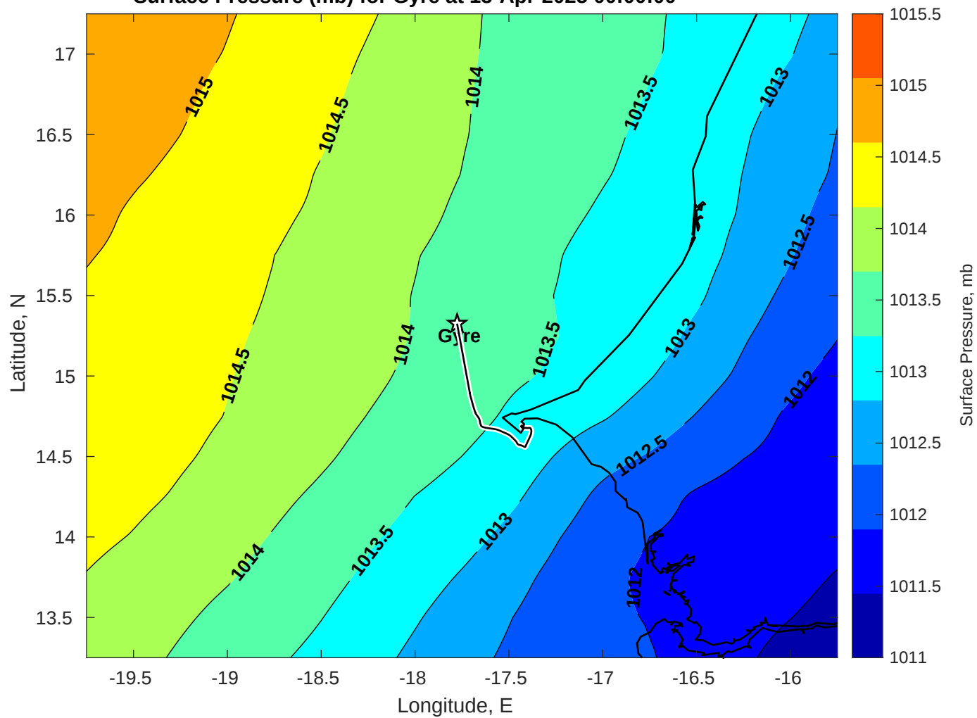
Surface Pressure (mb) for Gyre at 13-Apr-2025 00:00:00
