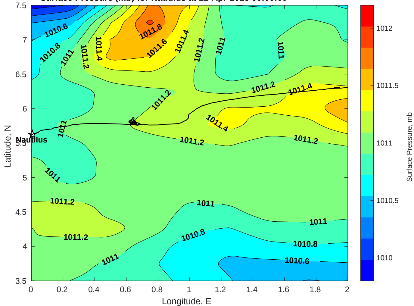
Surface Pressure (mb) for Nautilus at 11-Apr-2025 00:00:00
