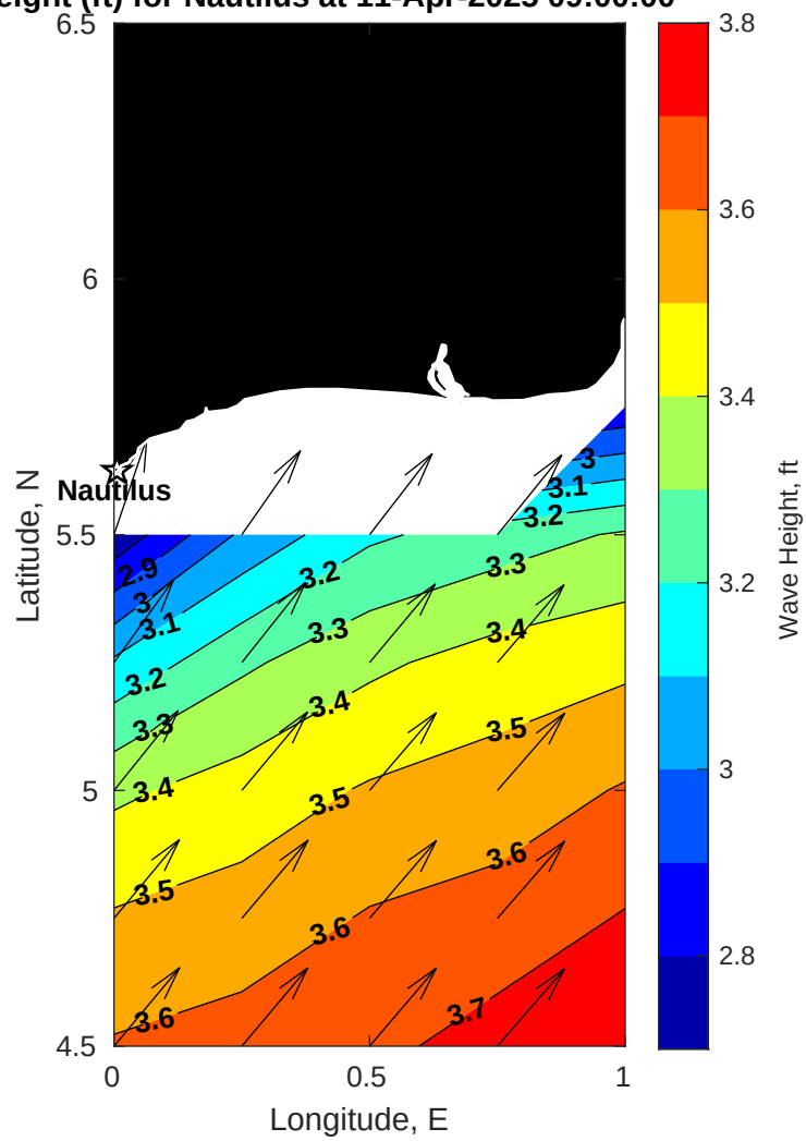
Wave Height (ft) for Nautilus at 11-Apr-2025 09:00:00
