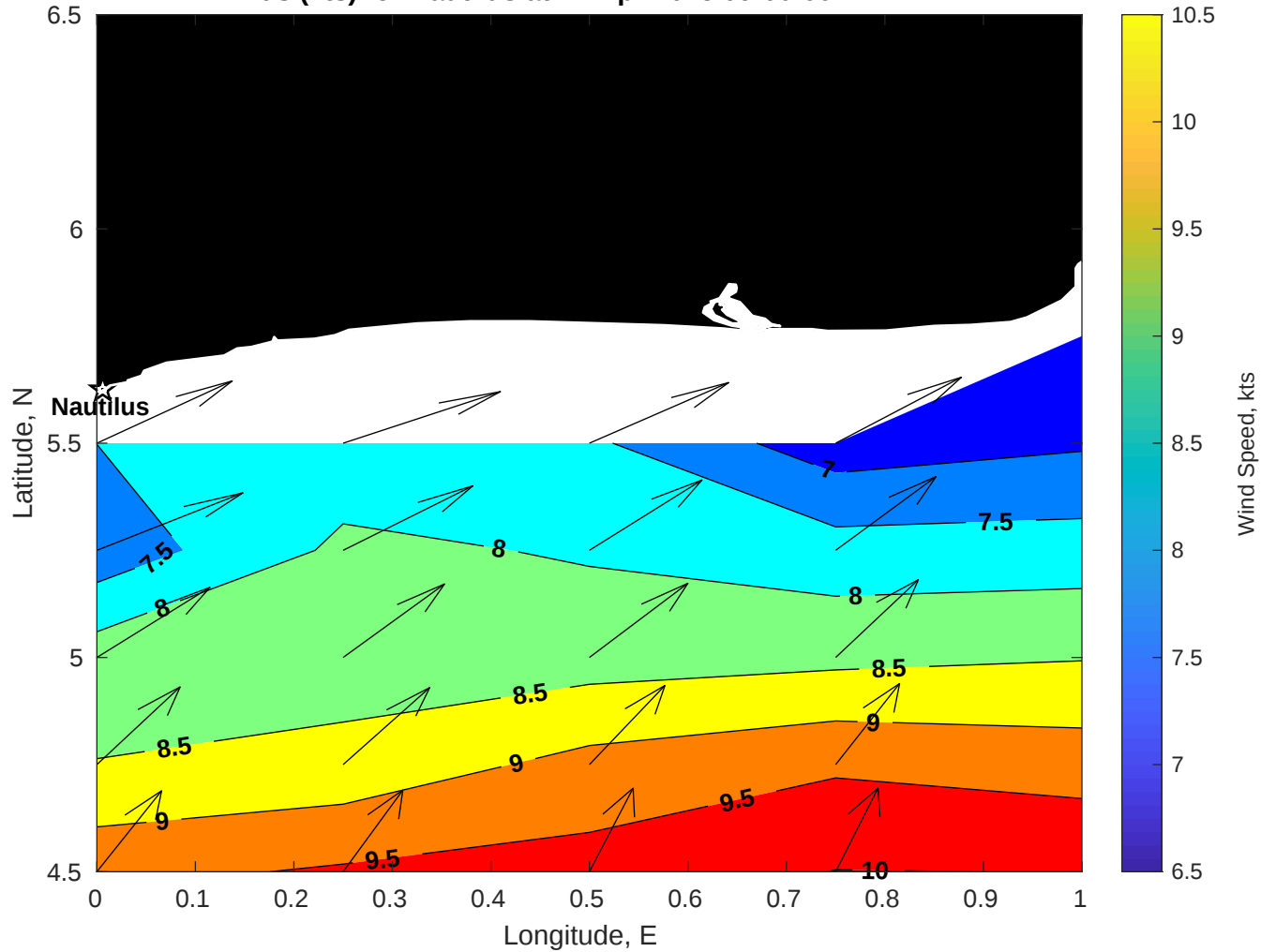
Winds (kts) for Nautilus at 11-Apr-2025 09:00:00
