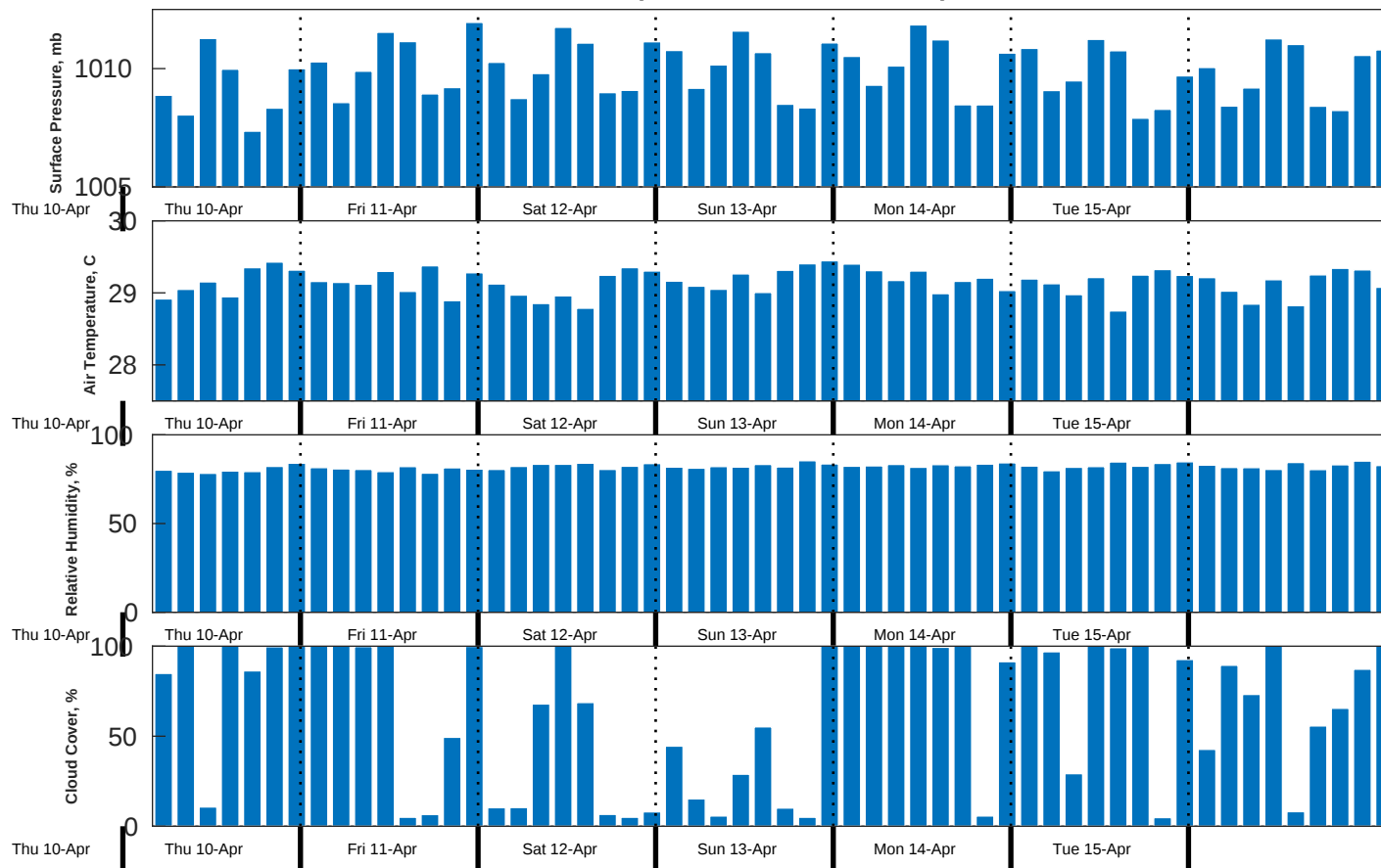
Met Forecast for Nautilus from 11-Apr-2025 00:00:00 to 18-Apr-2025 00:00:00
