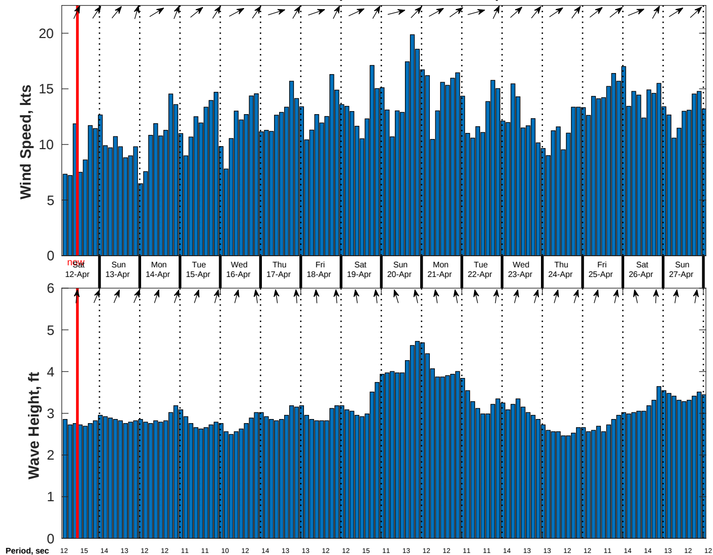
Wind & Wave Forecast for Nautilus from 11-Apr-2025 02:00:00 to 27-Apr-2025 02:00:00
