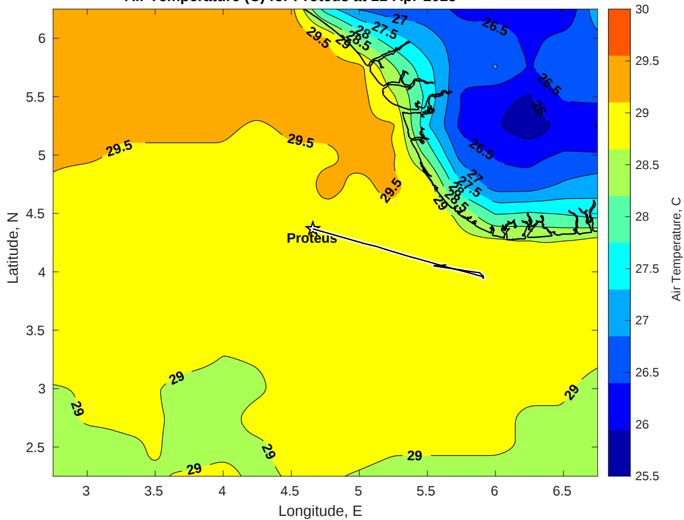
Air Temperature (C) for Proteus at 11-Apr-2025
