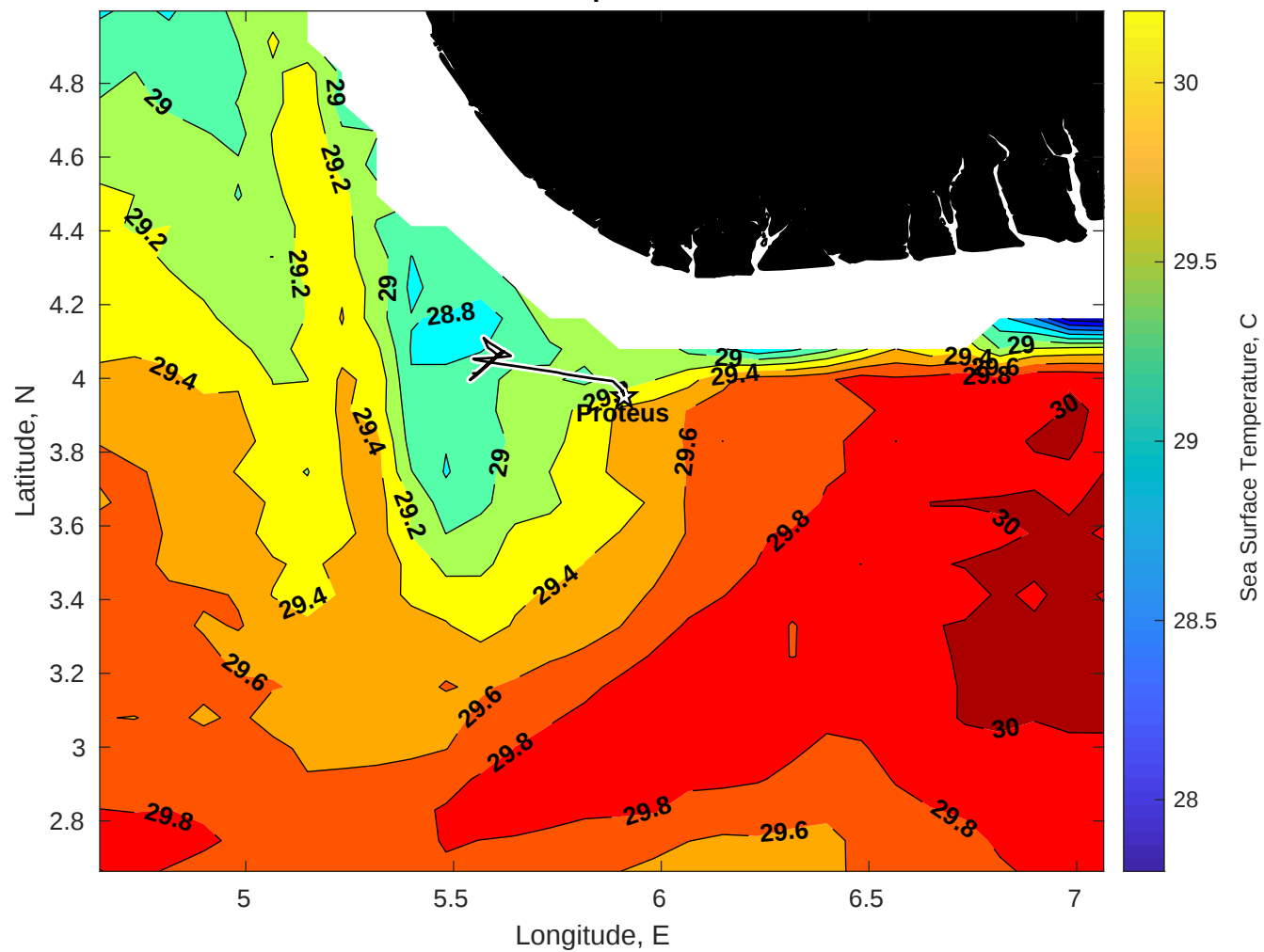
SST for Proteus at 10-Apr-2025 00:00:00
