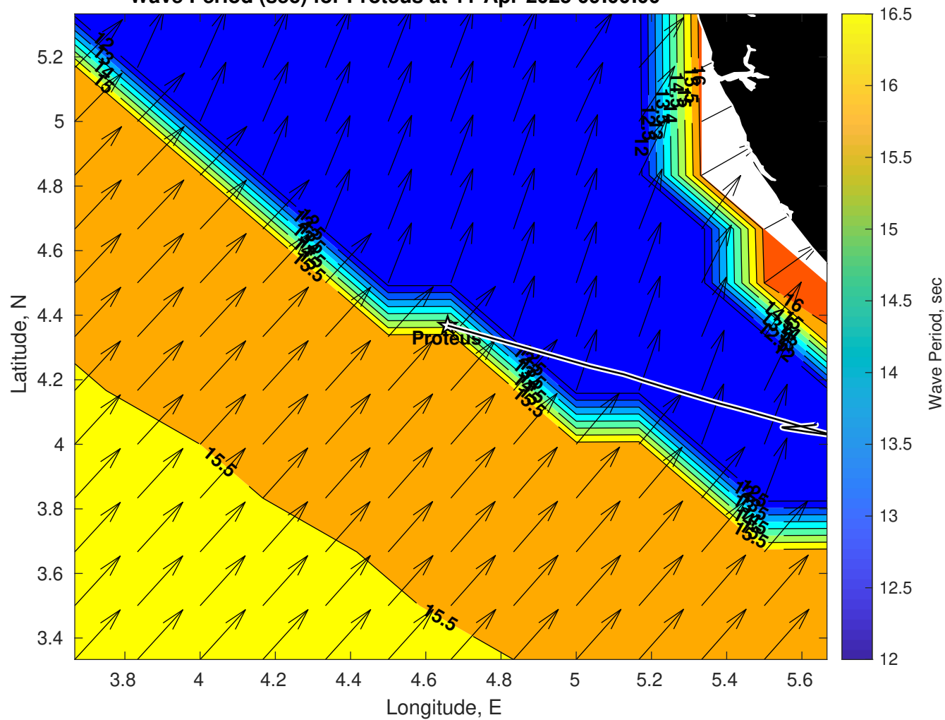
Wave Period (sec) for Proteus at 11-Apr-2025 09:00:00
