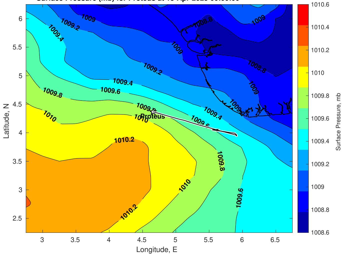
Surface Pressure (mb) for Proteus at 13-Apr-2025 00:00:00
