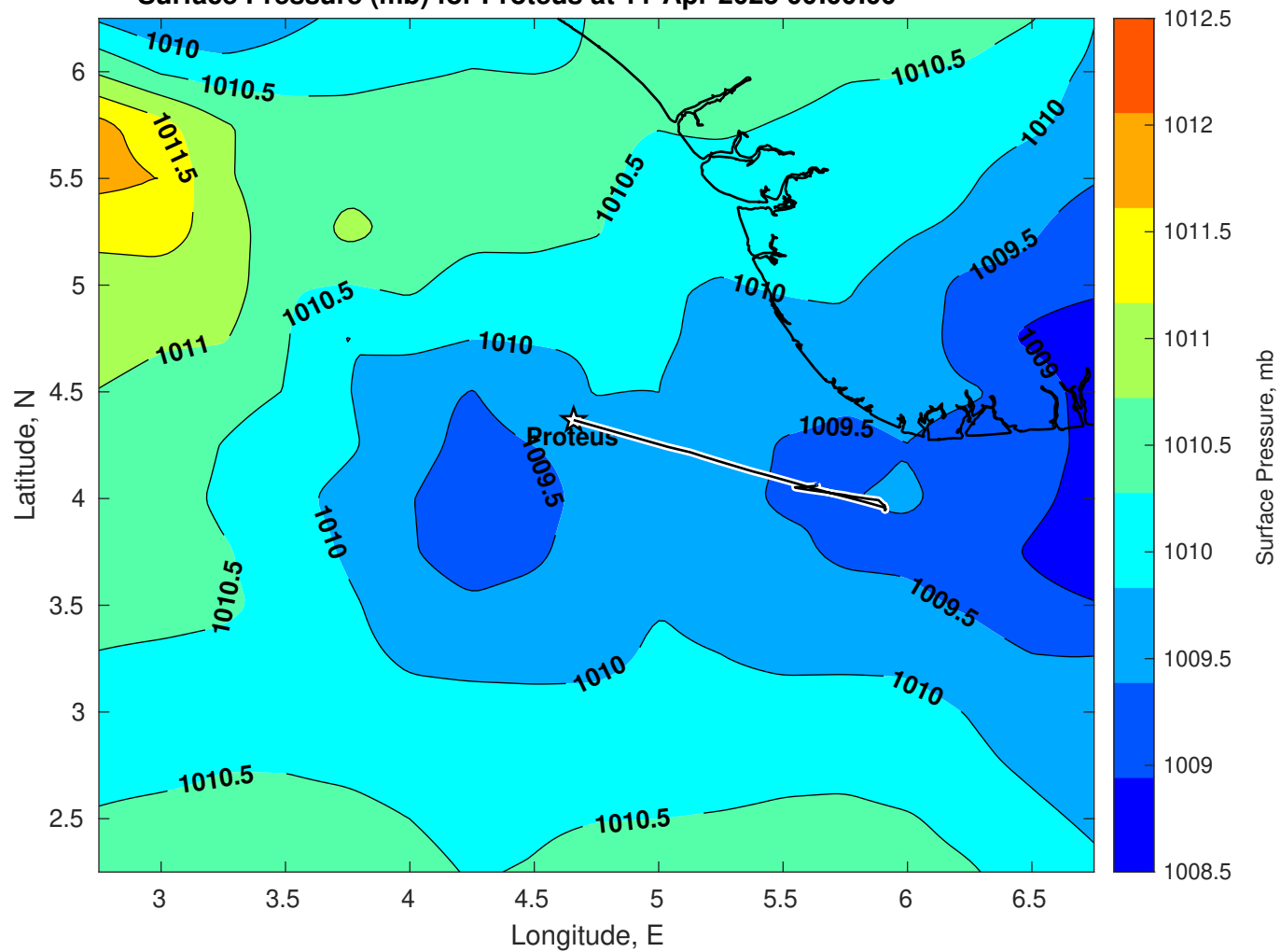
Surface Pressure (mb) for Proteus at 11-Apr-2025 00:00:00
