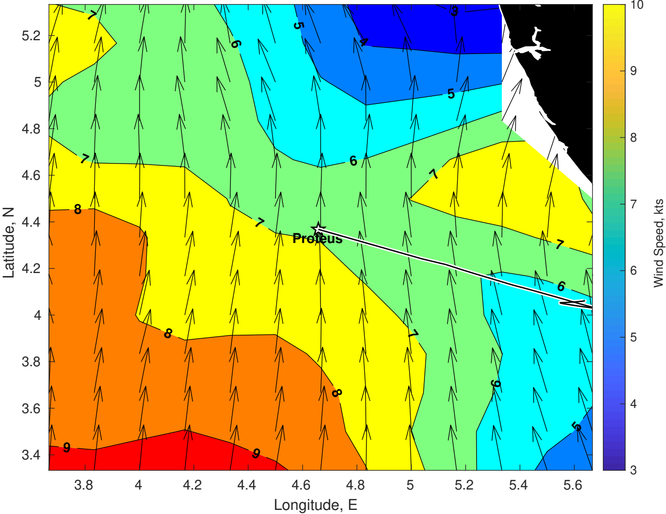
Winds (kts) for Proteus at 11-Apr-2025 09:00:00
