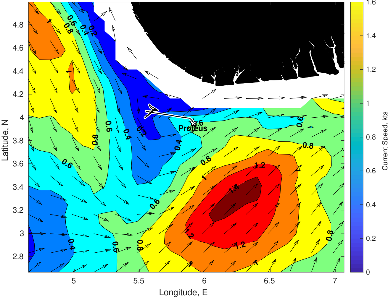
Surface Currents for Proteus at 10-Apr-2025 00:00:00
