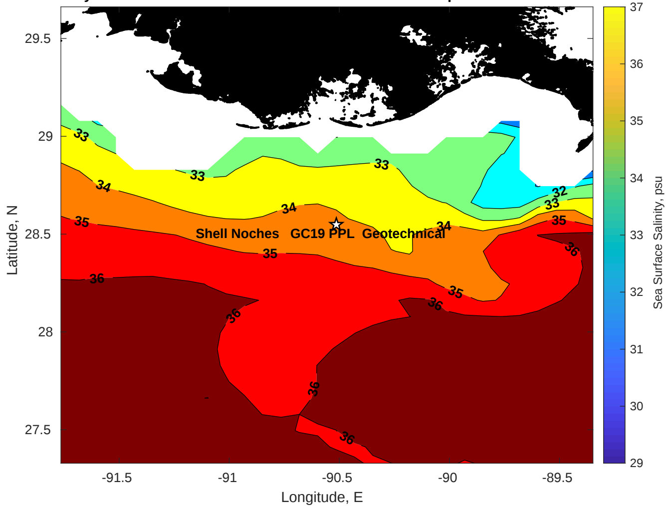
Surface Salinity for Shell Noches GC19 PPL Geotechnical at 10-Apr-2025 00:00:00
