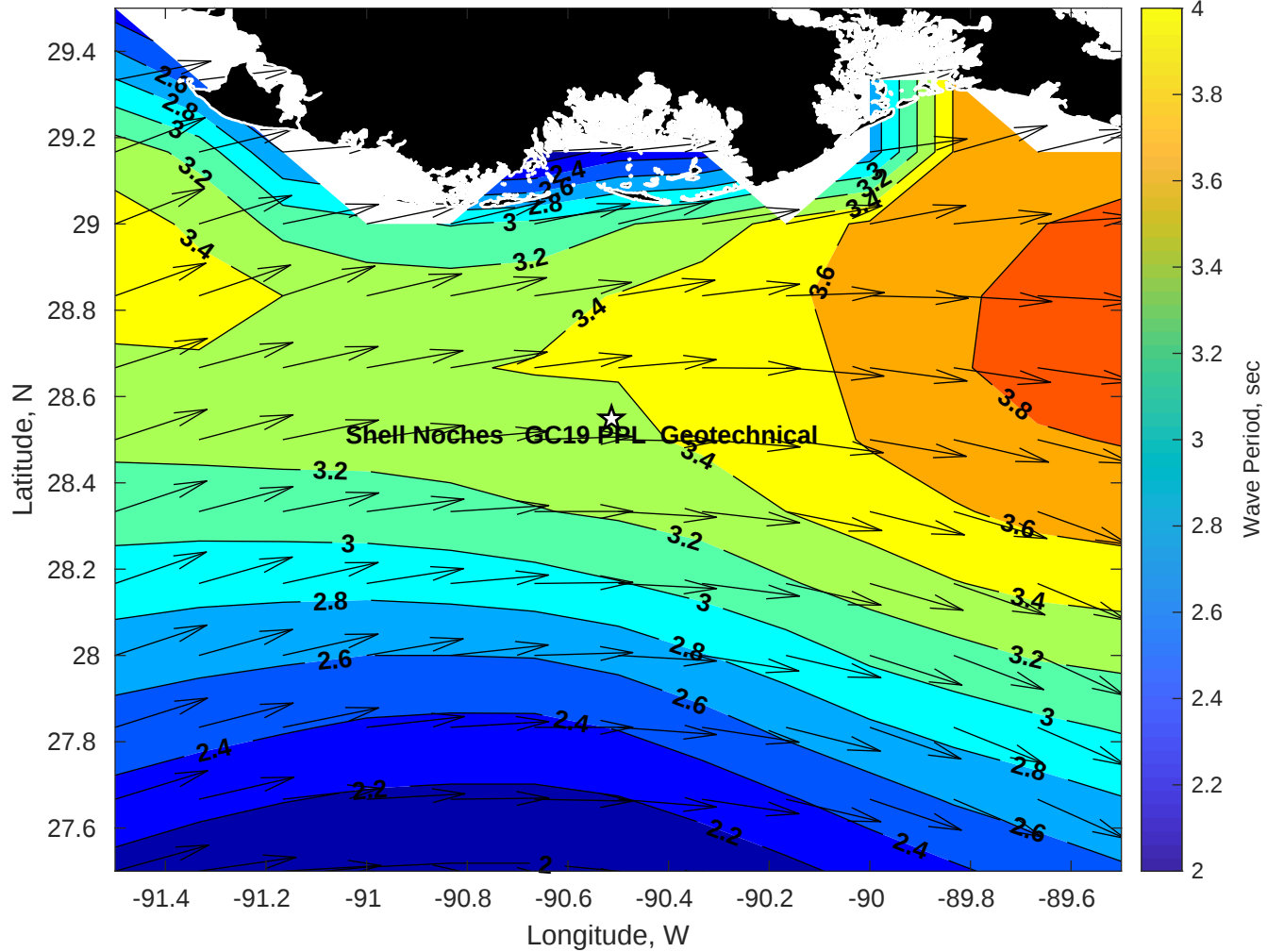
Wave Period (sec) for Shell Noches GC19 PPL Geotechnical at 11-Apr-2025 09:00:00
