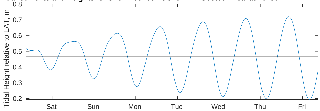
Tidal Currents and Heights for Shell Noches GC19 PPL Geotechnical at 20250411
