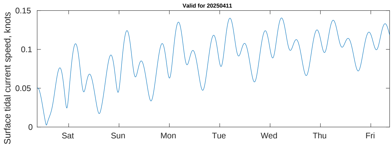
Tidal Currents and Heights for Shell Noches GC19 PPL Geotechnical at 20250411
