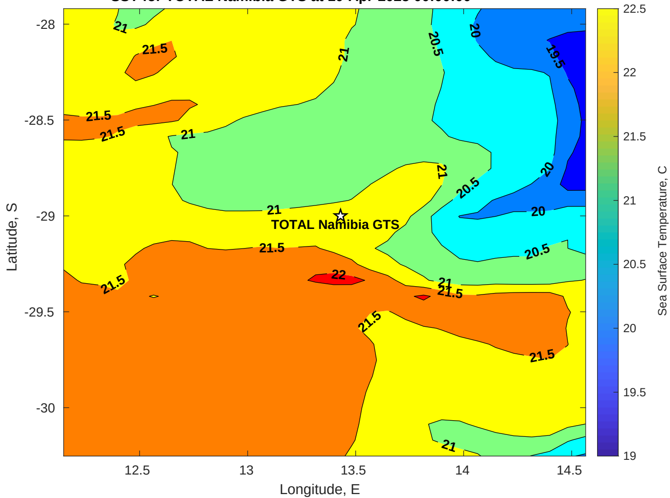
SST for TOTAL Namibia GTS at 10-Apr-2025 00:00:00
