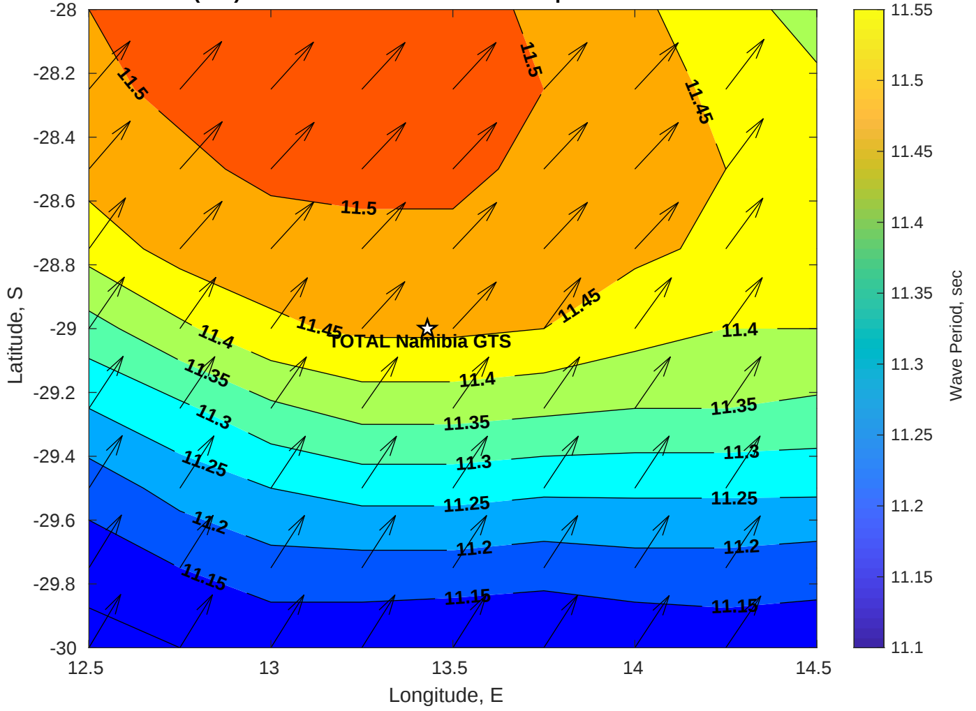
Wave Period (sec) for TOTAL Namibia GTS at 11-Apr-2025 09:00:00
