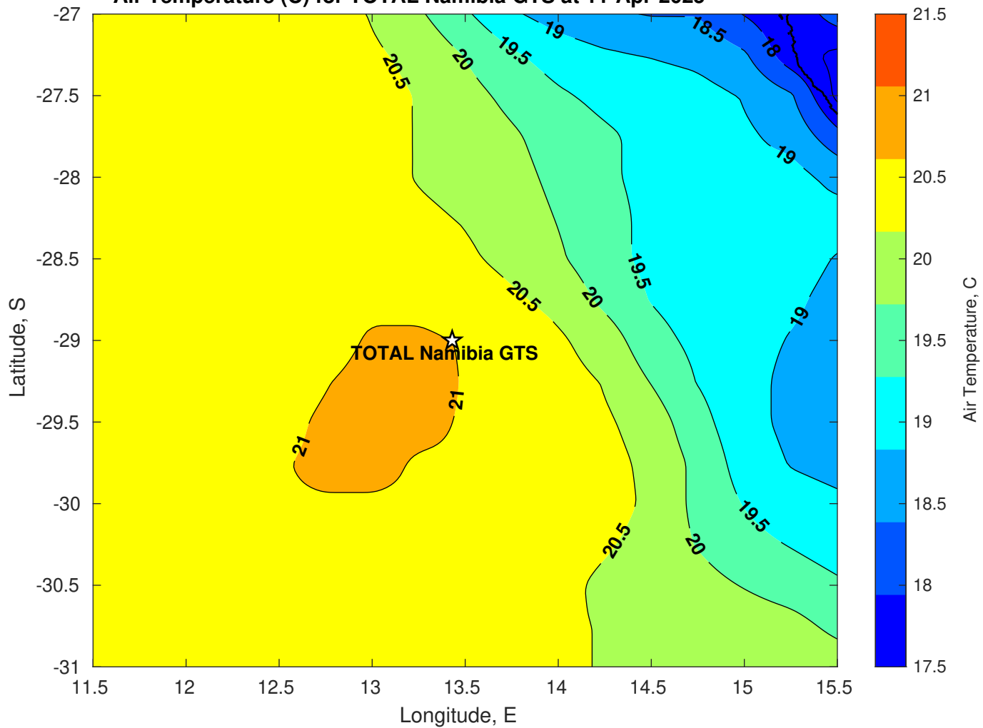
Air Temperature (C) for TOTAL Namibia GTS at 11-Apr-2025
