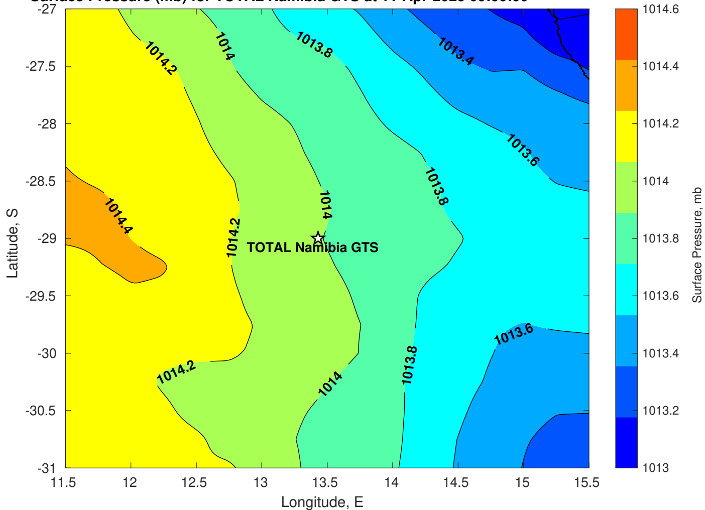
Surface Pressure (mb) for TOTAL Namibia GTS at 11-Apr-2025 00:00:00
