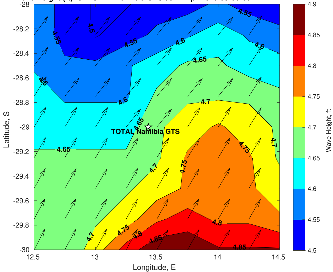
Wave Height (ft) for TOTAL Namibia GTS at 11-Apr-2025 09:00:00
