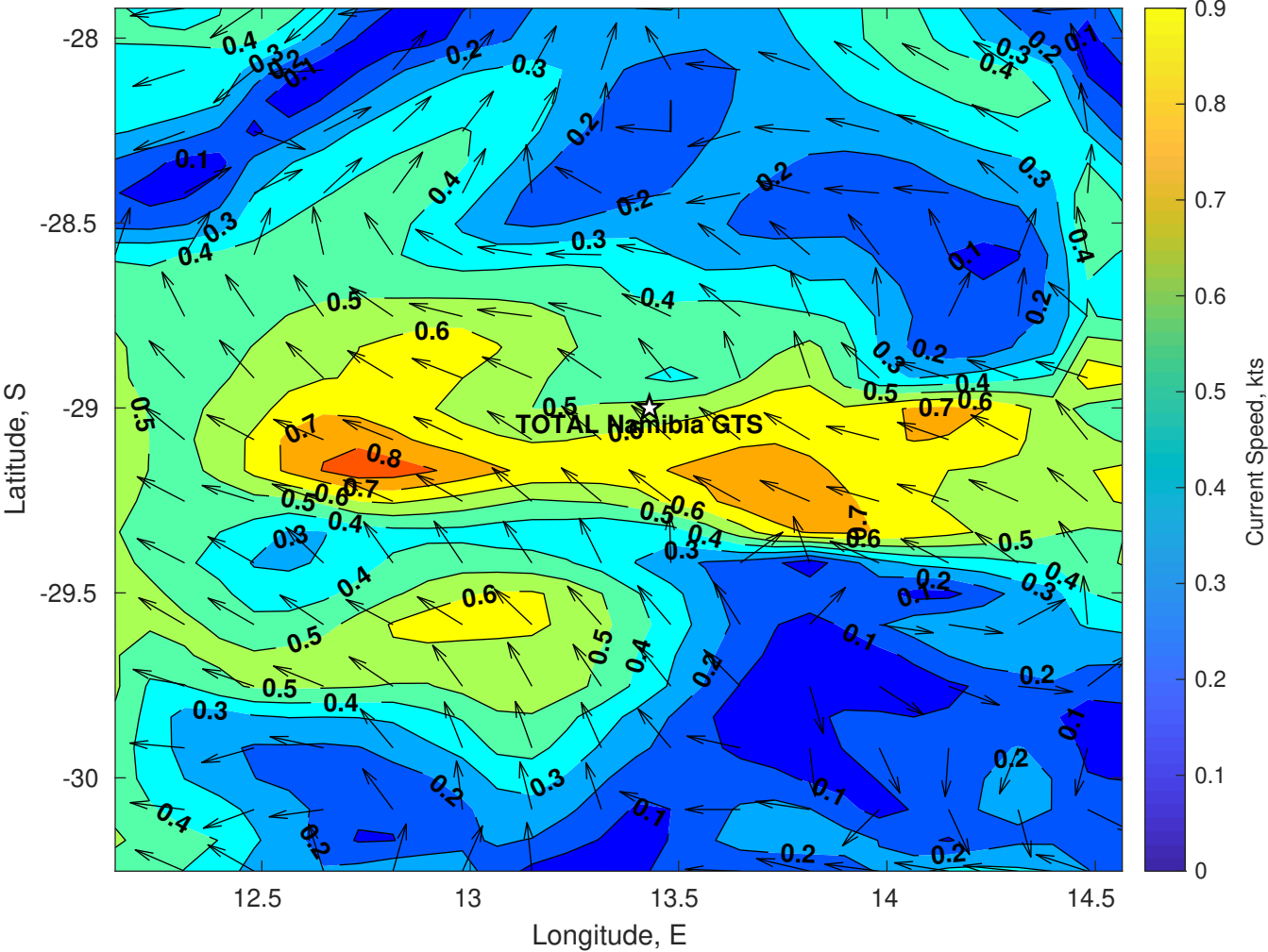
Surface Currents for TOTAL Namibia GTS at 10-Apr-2025 00:00:00
