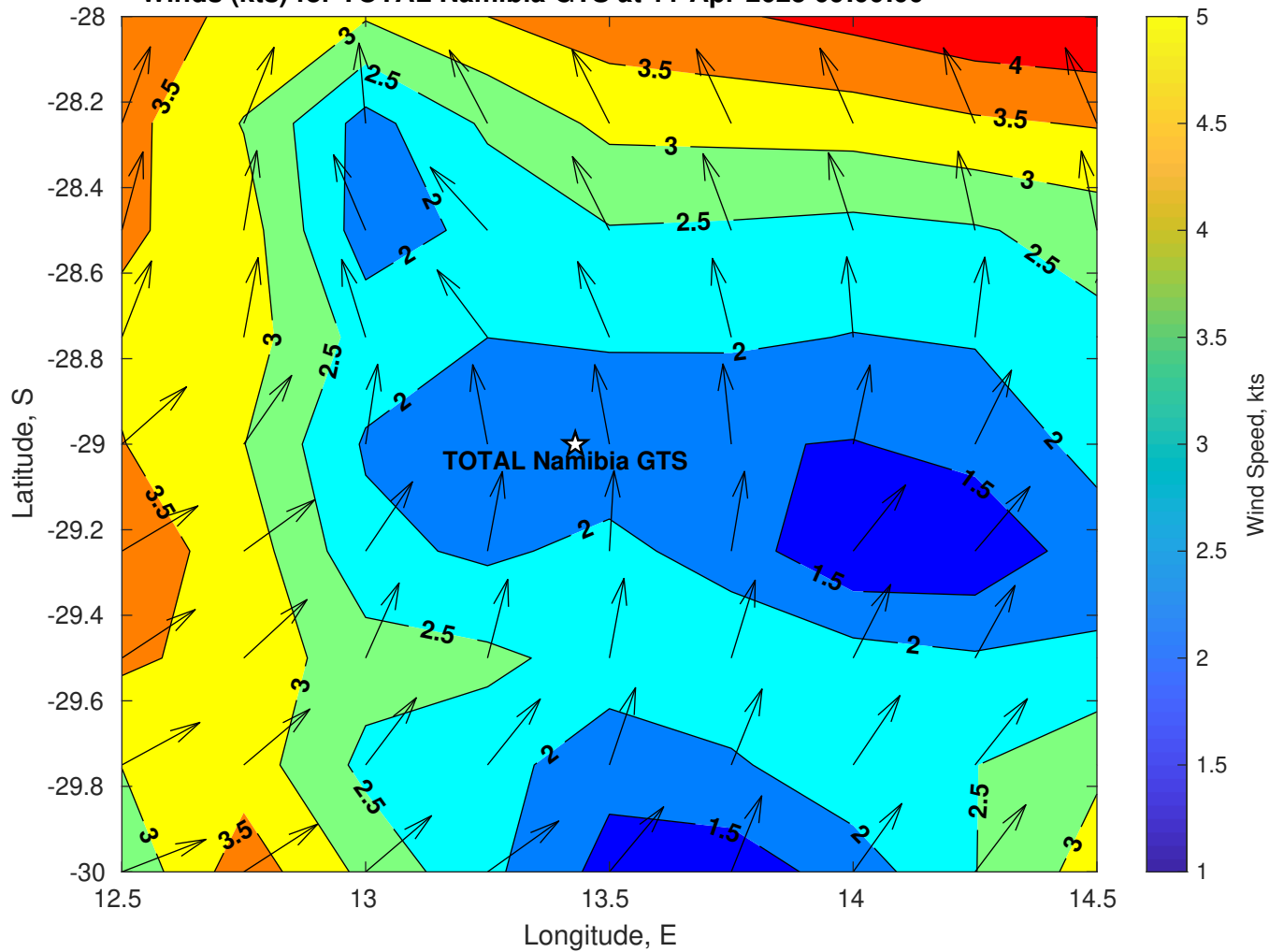
Winds (kts) for TOTAL Namibia GTS at 11-Apr-2025 09:00:00
