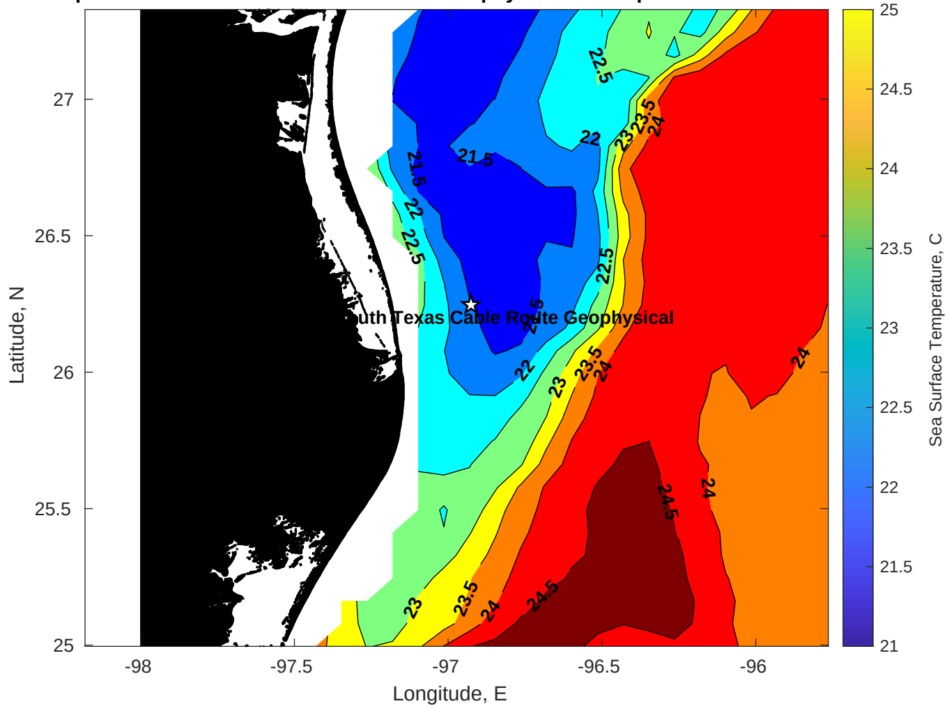
SST for Tampnet P2378 South Texas Cable Route Geophysical at 10-Apr-2025 00:00:00
