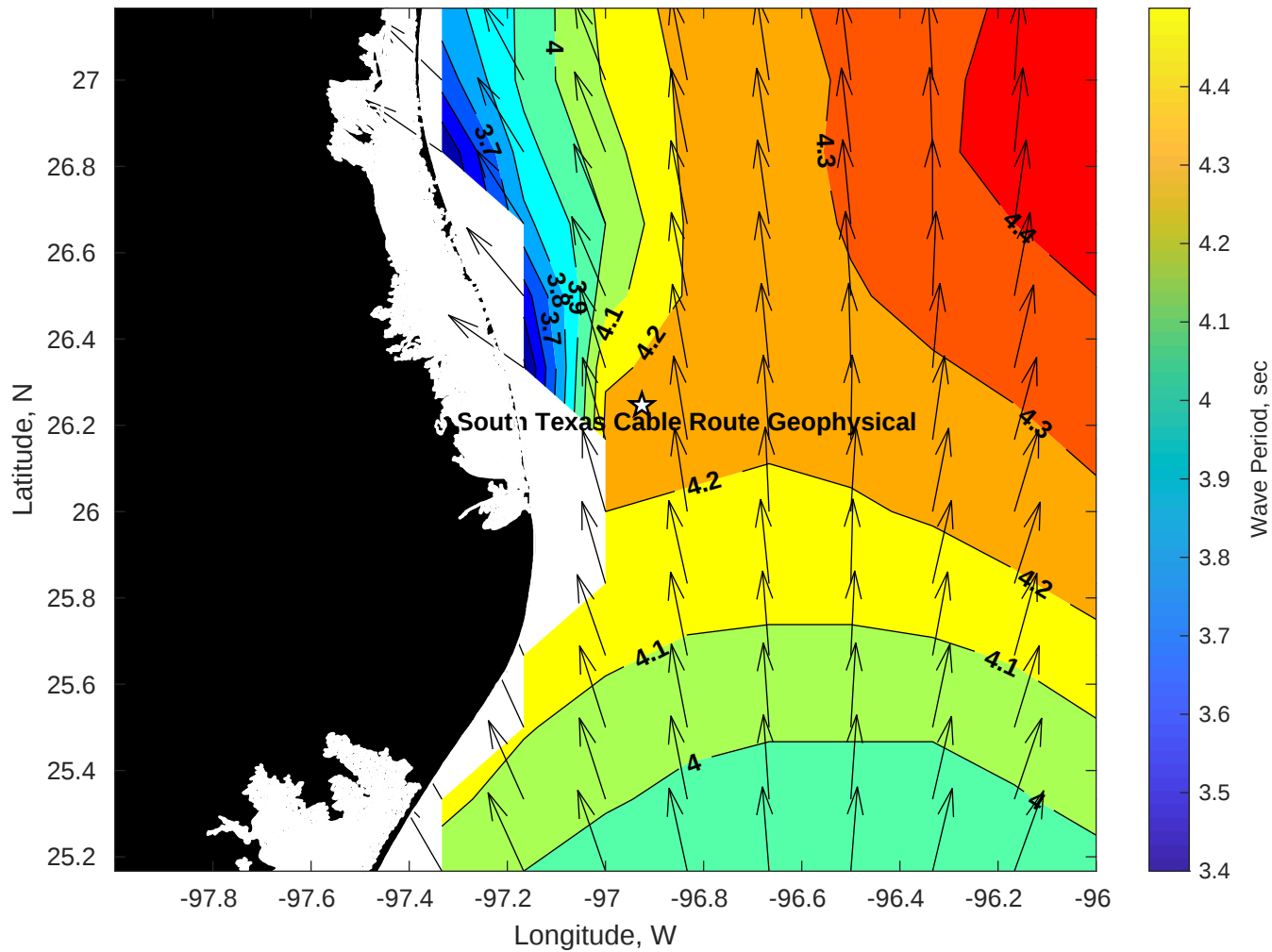
Period (sec) for Tampnet P2378 South Texas Cable Route Geophysical at 11-Apr-2025 09:00:00
