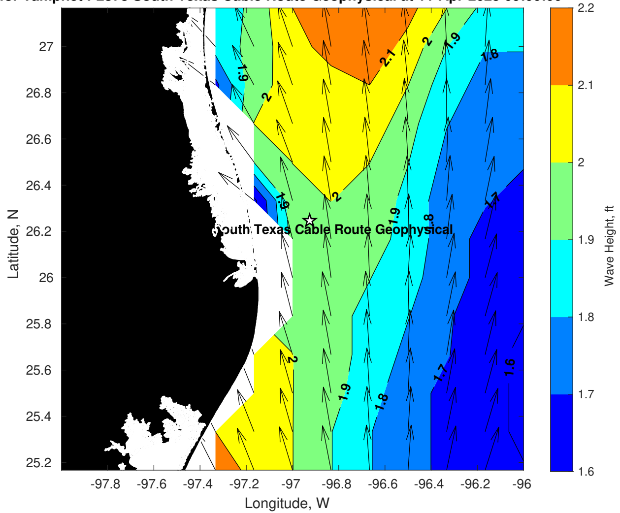
Wave Height (ft) for Tampnet P2378 South Texas Cable Route Geophysical at 11-Apr-2025 09:00:00
