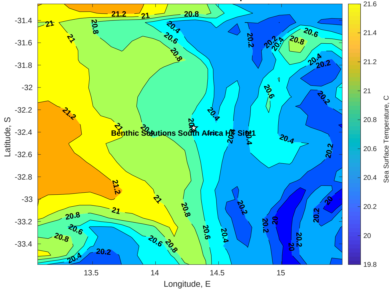
SST for Benthic Solutions South Africa HF Site1 at 11-Apr-2025 00:00:00
