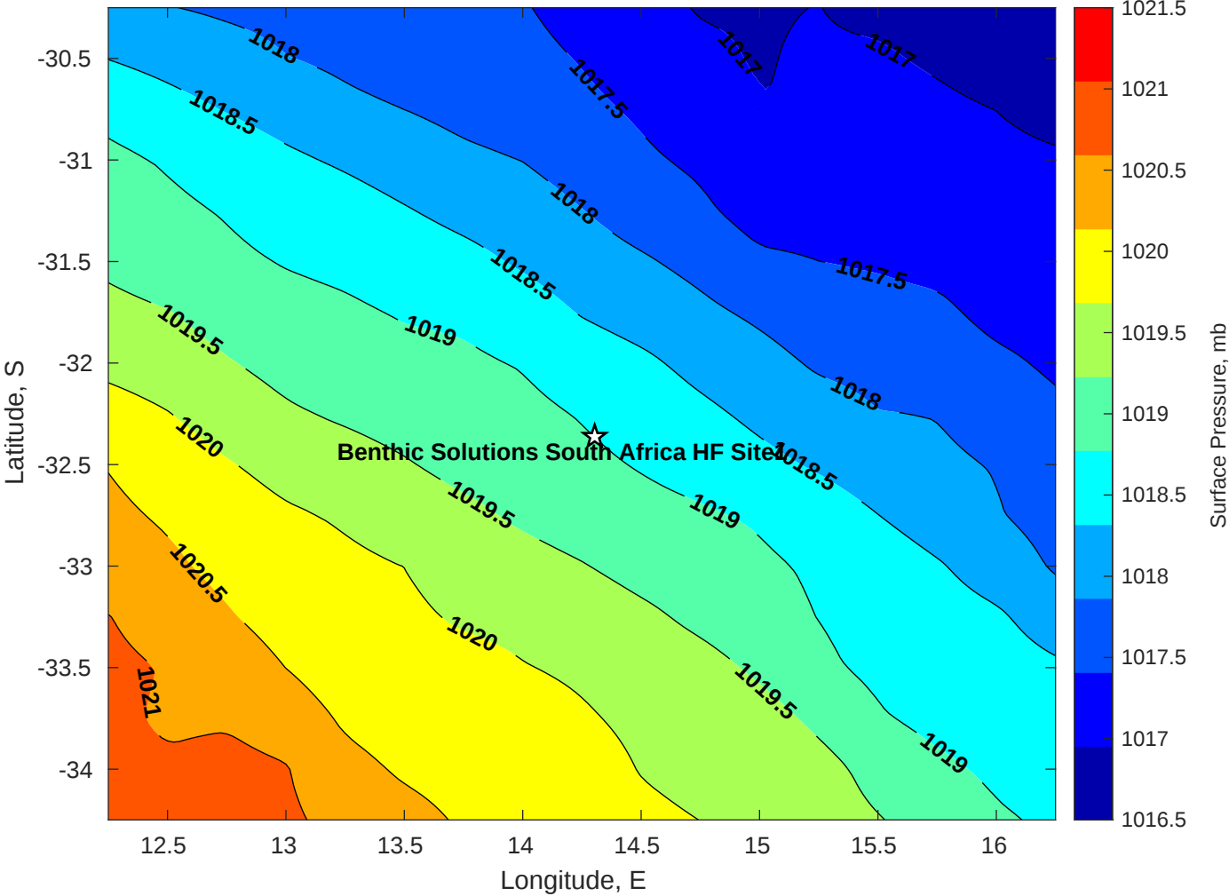
Surface Pressure (mb) for Benthic Solutions South Africa HF Site1 at 13-Apr-2025 00:00:00
