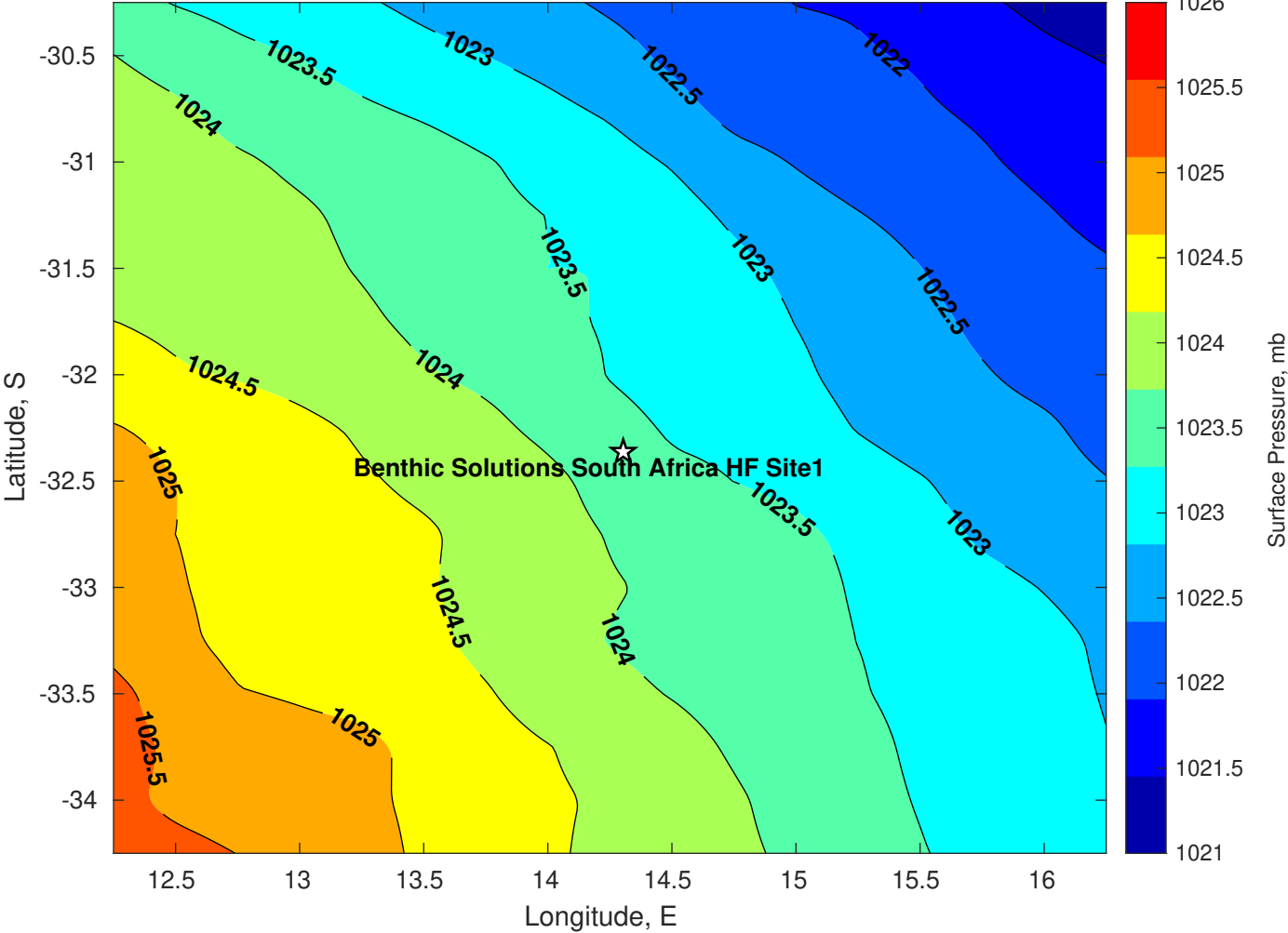
Surface Pressure (mb) for Benthic Solutions South Africa HF Site1 at 14-Apr-2025 00:00:00
