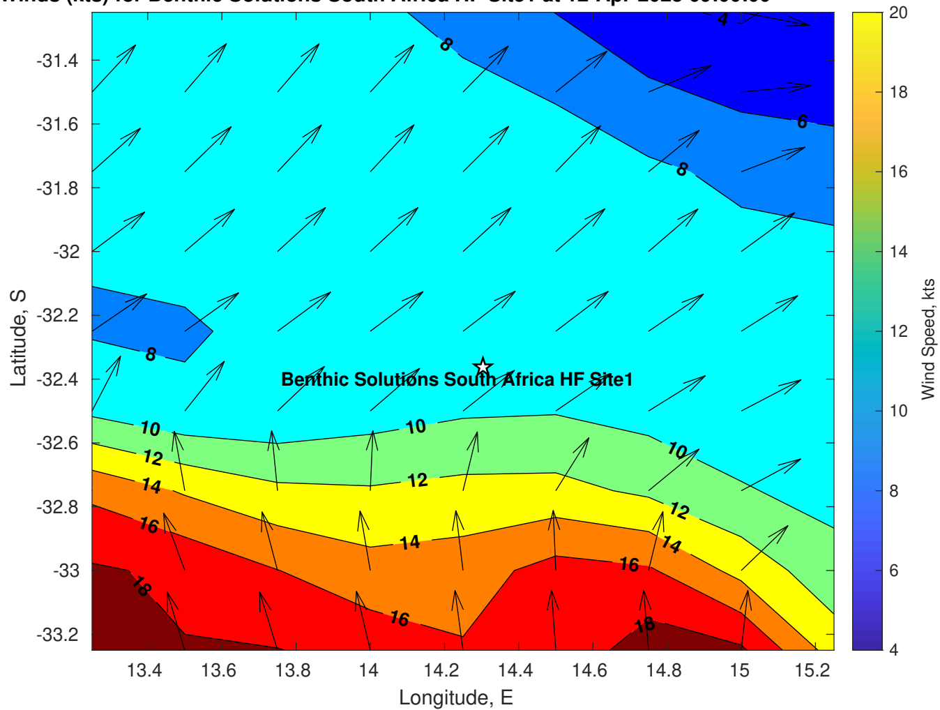
Winds (kts) for Benthic Solutions South Africa HF Site1 at 12-Apr-2025 09:00:00
