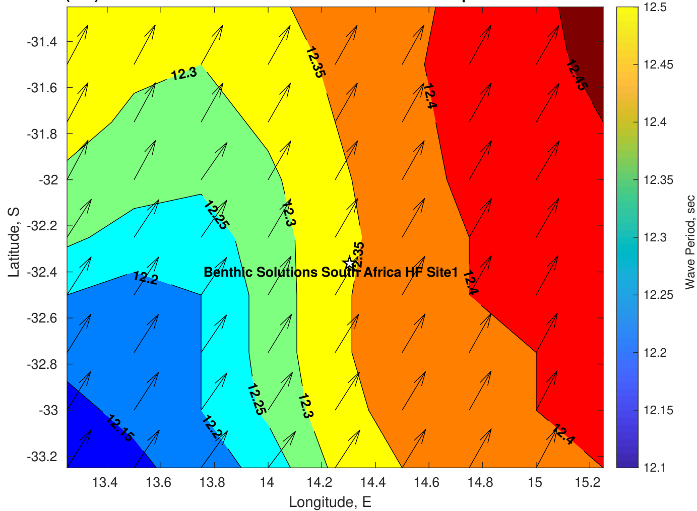
Wave Period (sec) for Benthic Solutions South Africa HF Site1 at 12-Apr-2025 09:00:00
