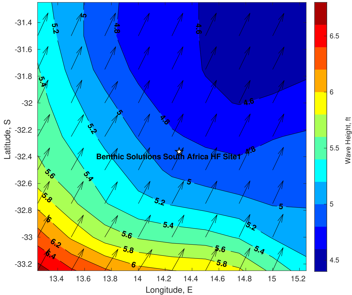
Wave Height (ft) for Benthic Solutions South Africa HF Site1 at 12-Apr-2025 09:00:00
