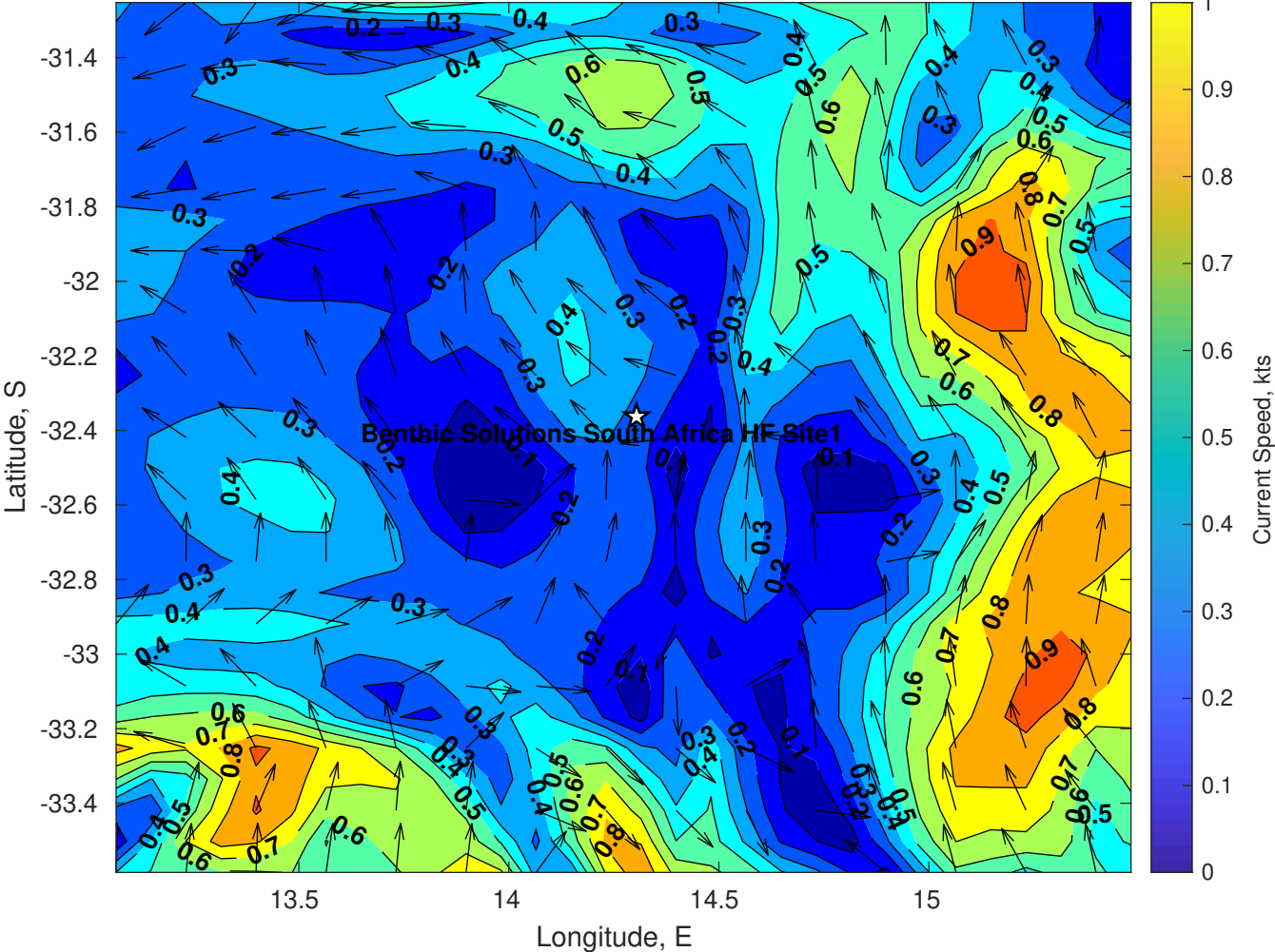
Surface Currents for Benthic Solutions South Africa HF Site1 at 11-Apr-2025 00:00:00
