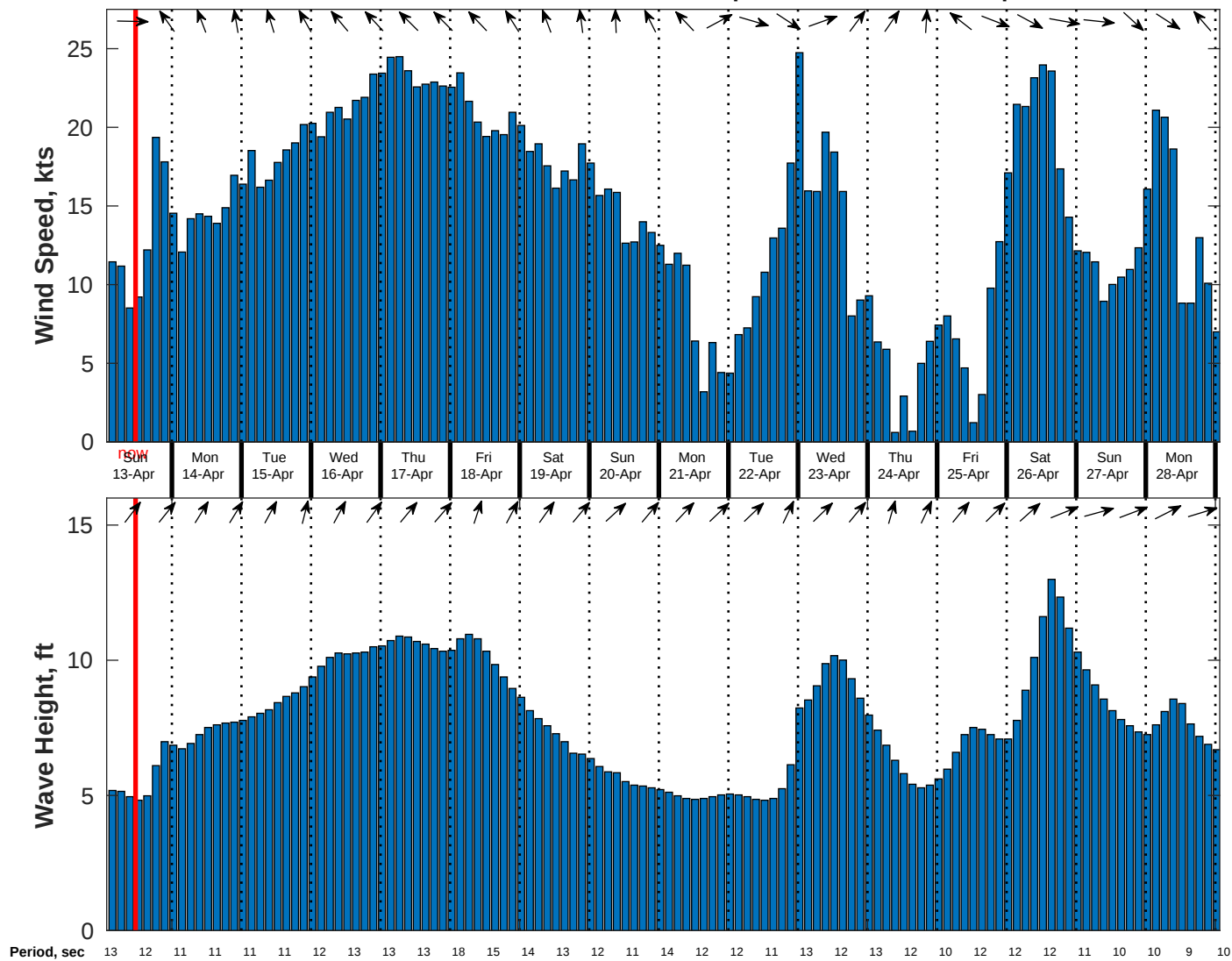
Wind & Wave Forecast for Benthic Solutions South Africa HF Site1 from 12-Apr-2025 02:00:00 to 28-Apr-2025 02:00:00
