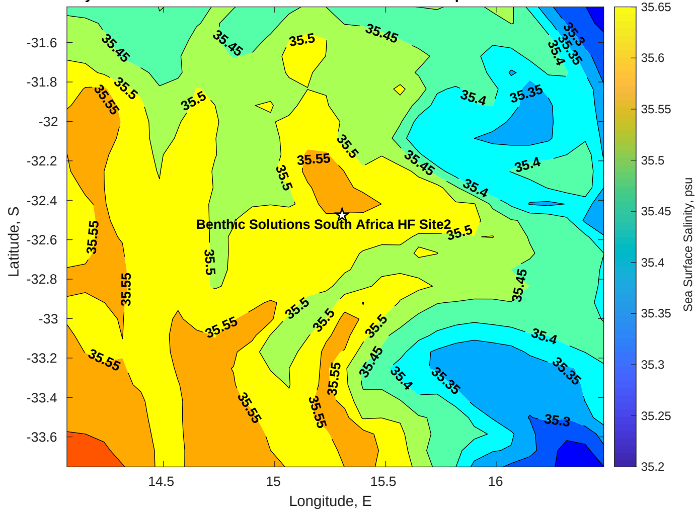
Surface Salinity for Benthic Solutions South Africa HF Site2 at 11-Apr-2025 00:00:00
