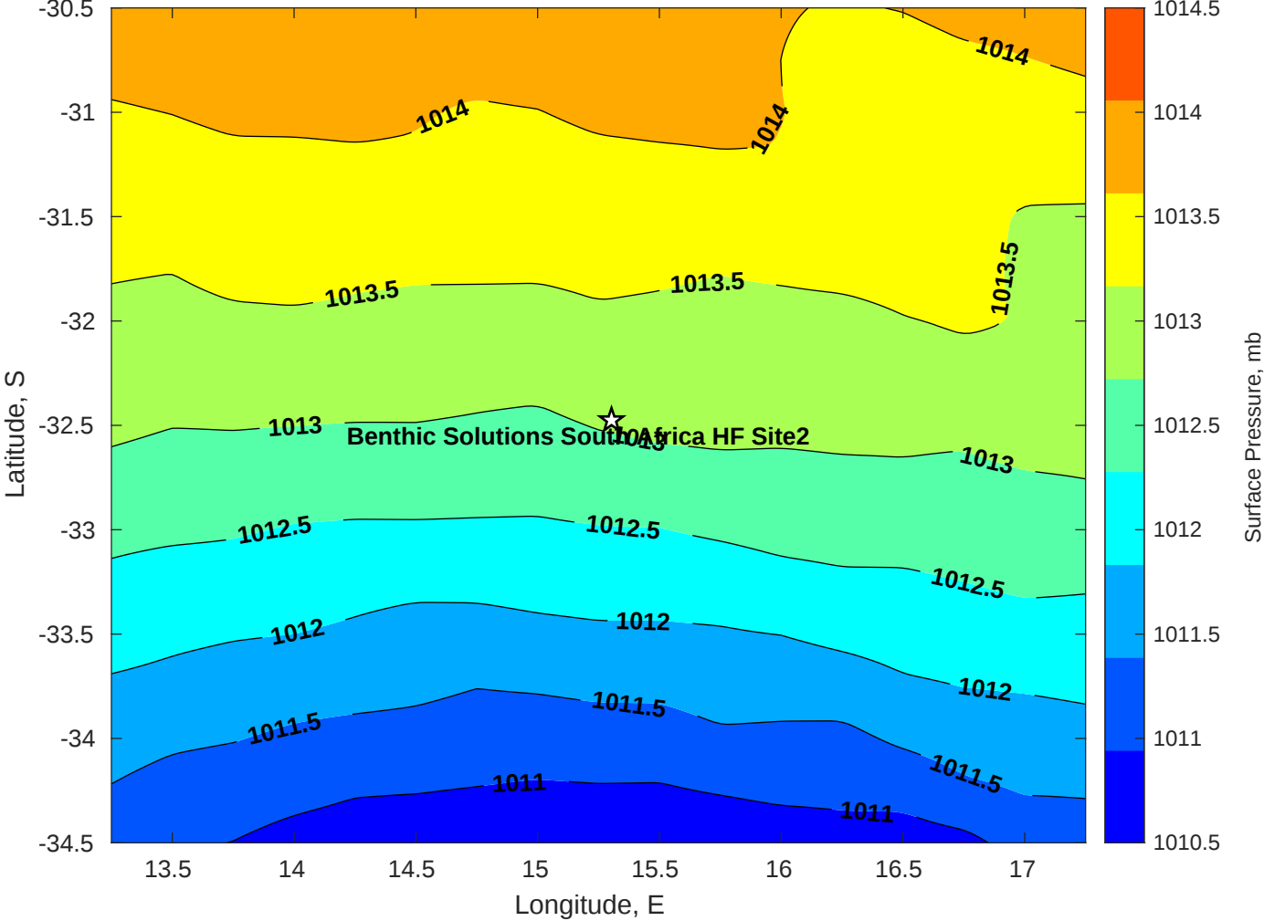
Surface Pressure (mb) for Benthic Solutions South Africa HF Site2 at 12-Apr-2025 00:00:00
