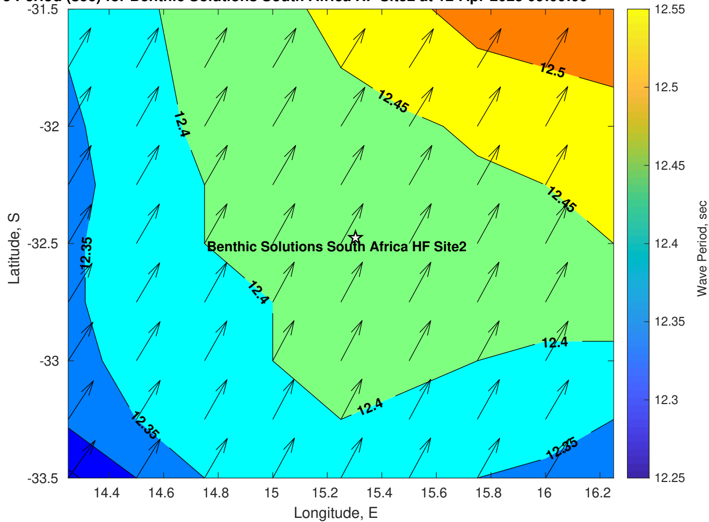
Wave Period (sec) for Benthic Solutions South Africa HF Site2 at 12-Apr-2025 09:00:00
