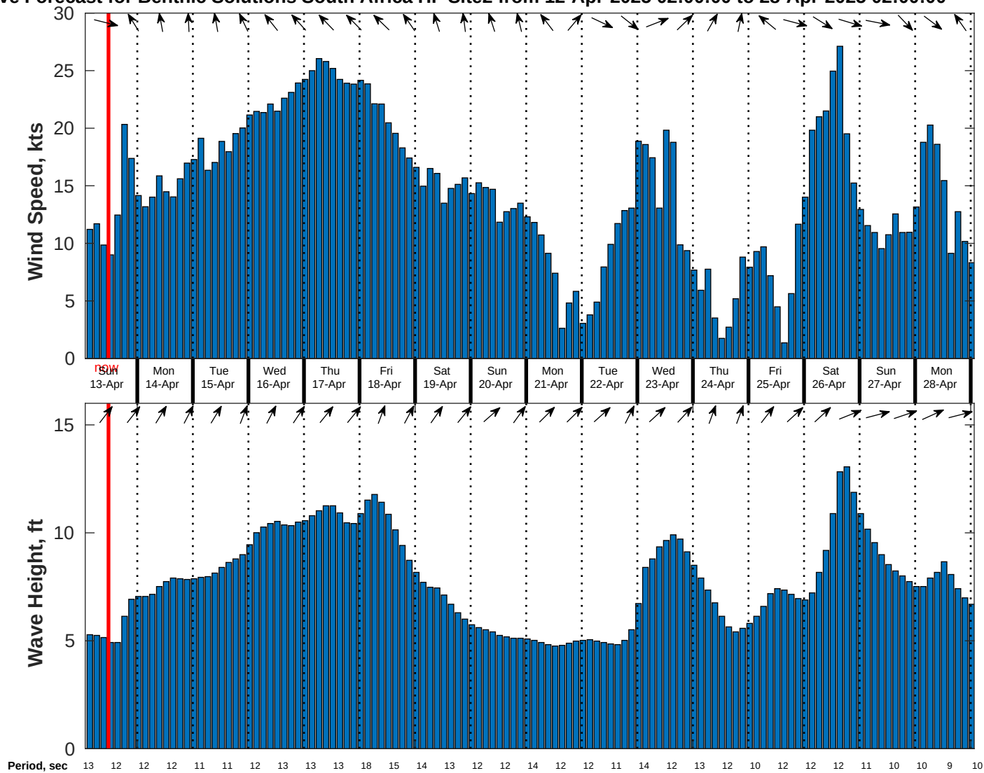
Wind & Wave Forecast for Benthic Solutions South Africa HF Site2 from 12-Apr-2025 02:00:00 to 28-Apr-2025 02:00:00
