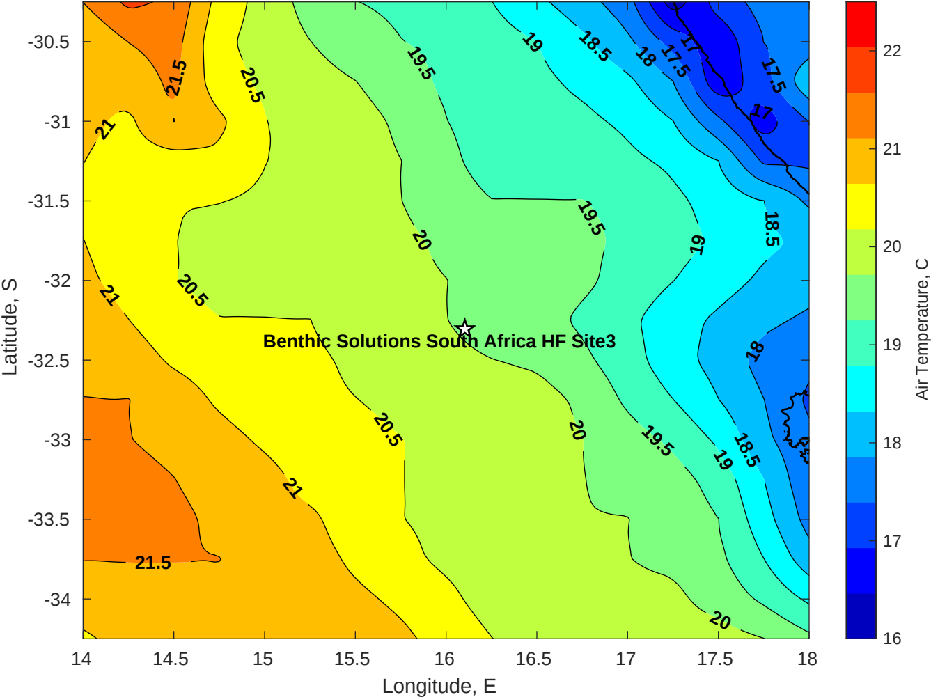
Air Temperature (C) for Benthic Solutions South Africa HF Site3 at 12-Apr-2025
