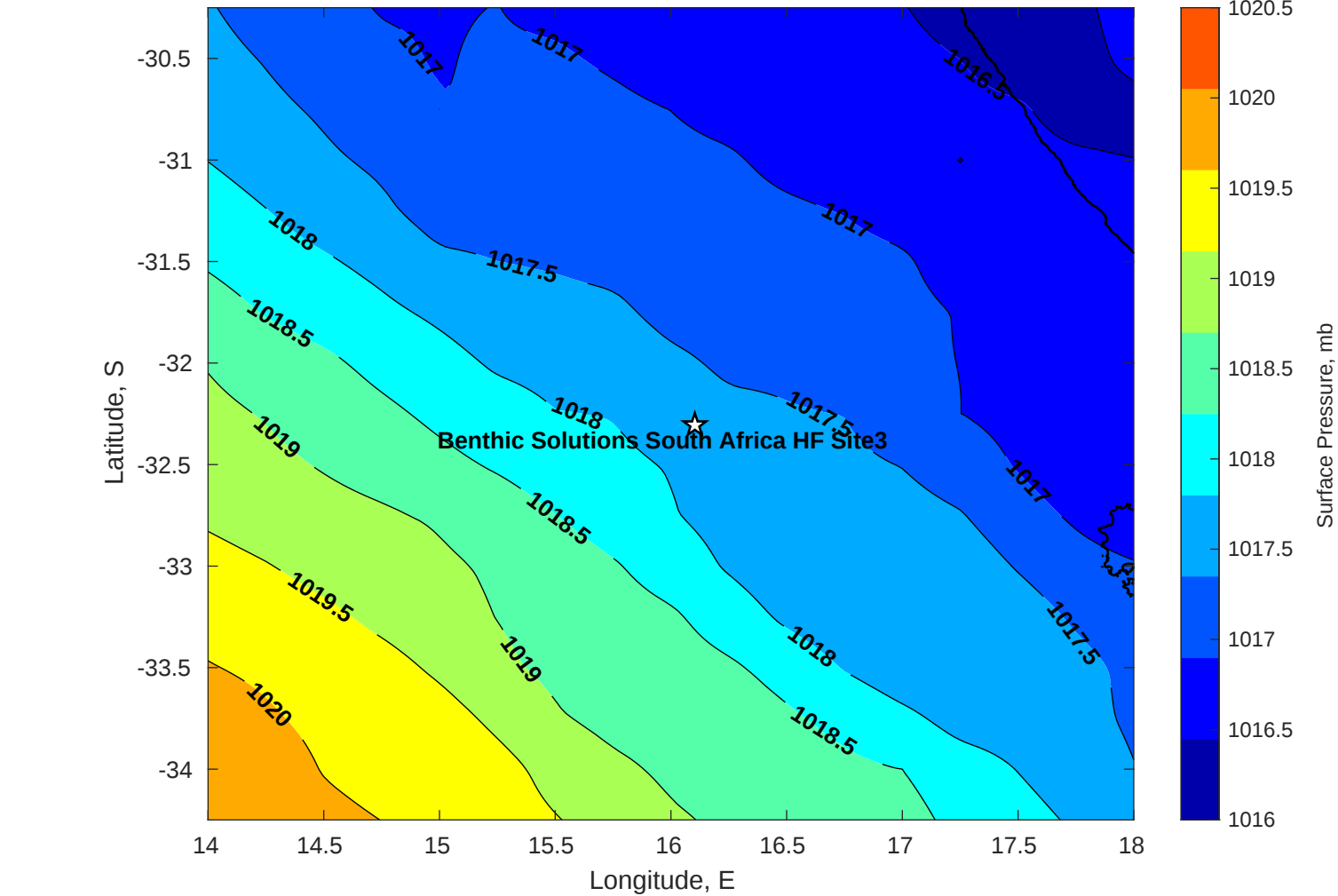
Surface Pressure (mb) for Benthic Solutions South Africa HF Site3 at 13-Apr-2025 00:00:00
