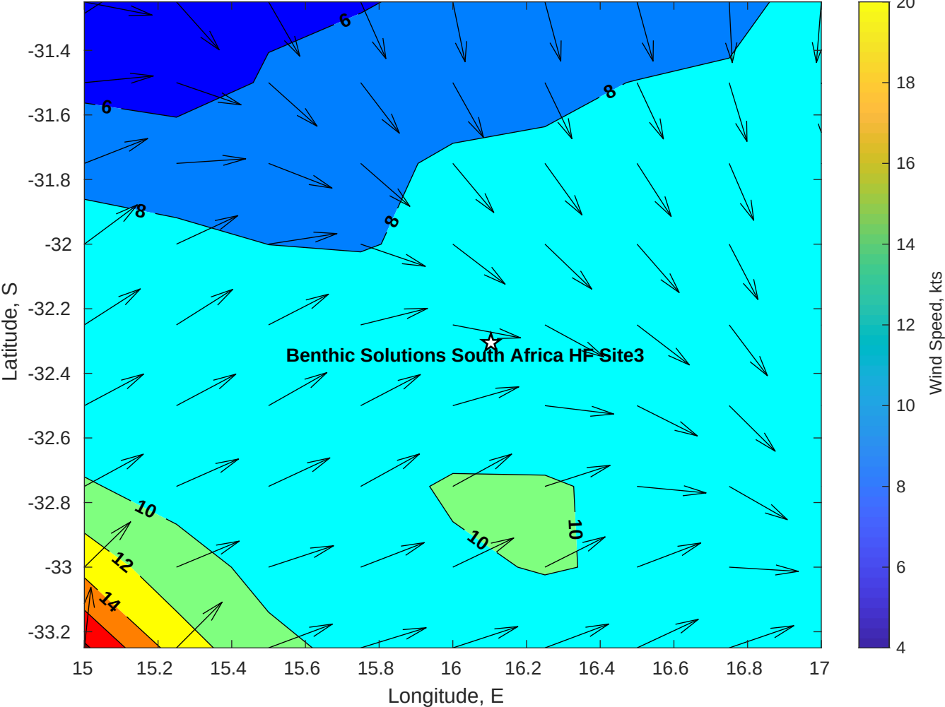
Winds (kts) for Benthic Solutions South Africa HF Site3 at 12-Apr-2025 09:00:00
