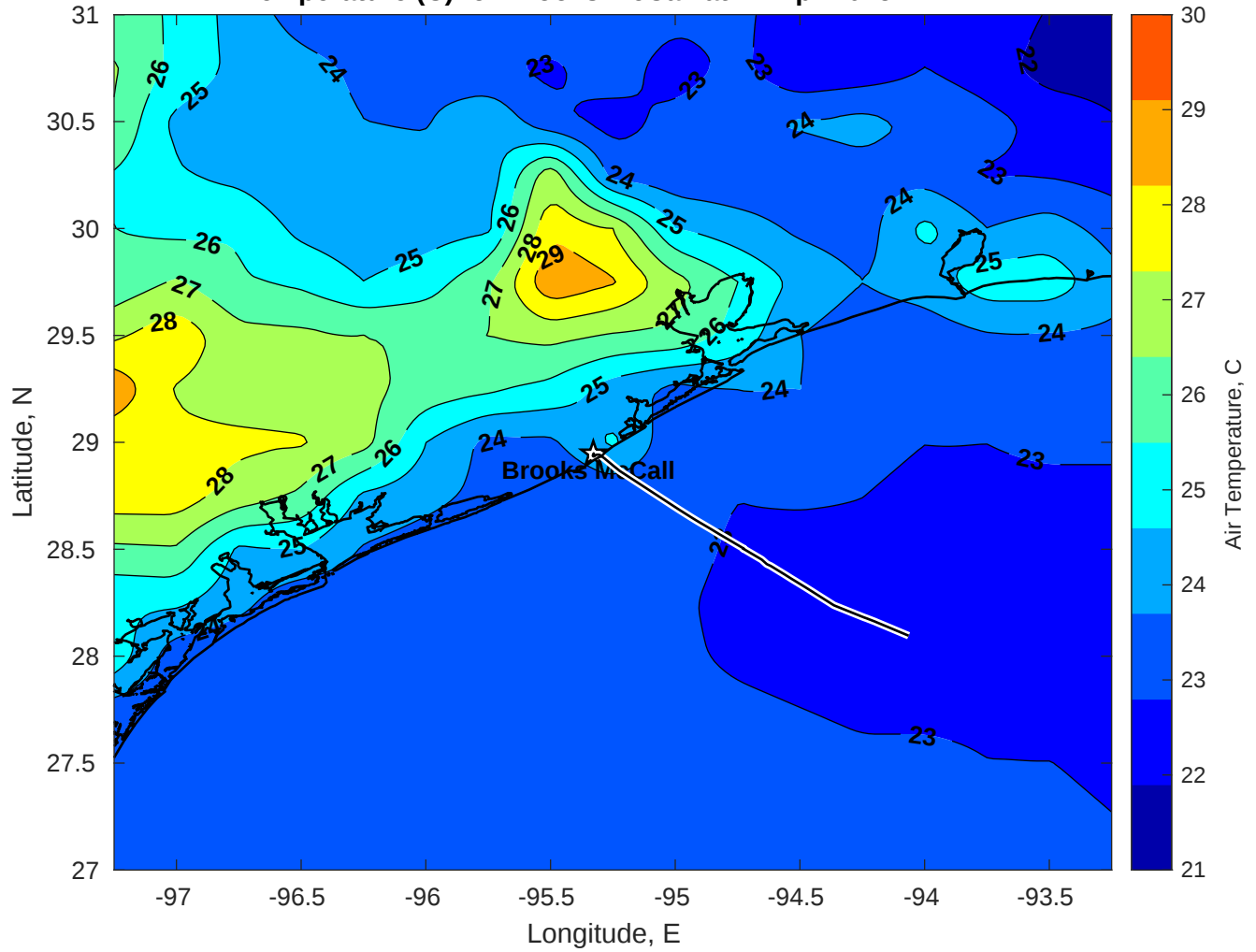
Air Temperature (C) for Brooks McCall at 12-Apr-2025
