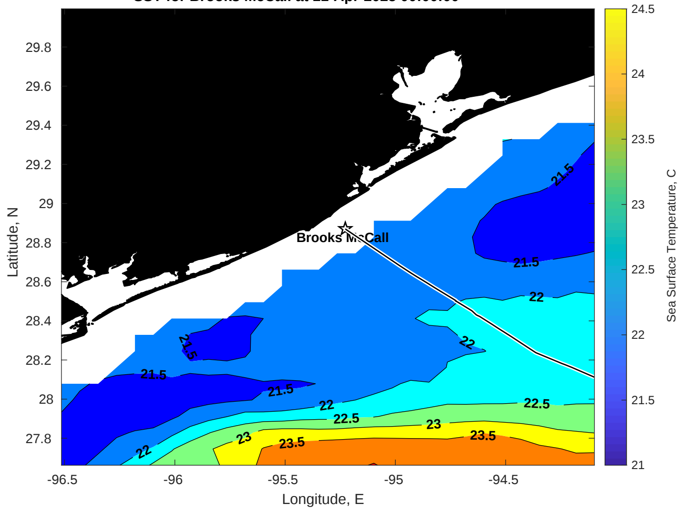
SST for Brooks McCall at 11-Apr-2025 00:00:00
