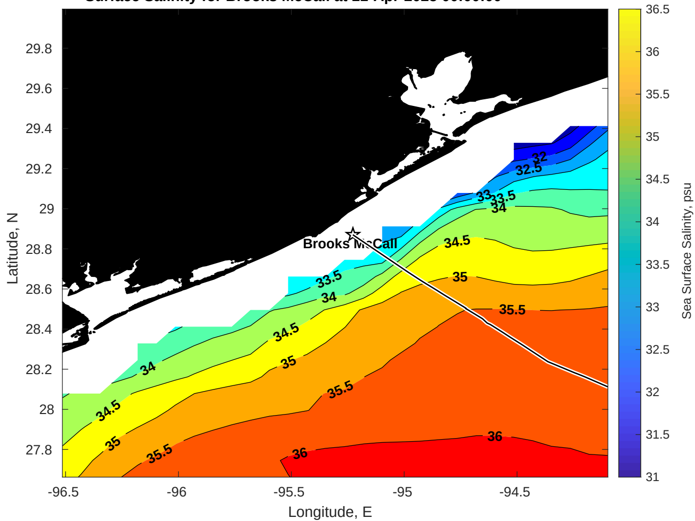
Surface Salinity for Brooks McCall at 11-Apr-2025 00:00:00
