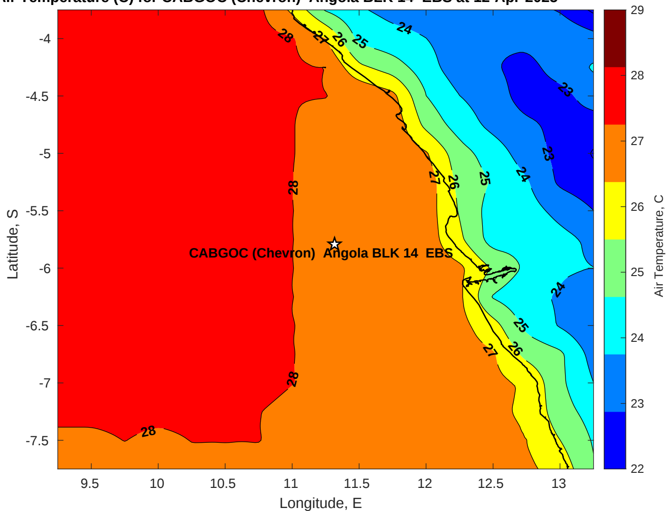
Air Temperature (C) for CABGOC (Chevron) Angola BLK 14 EBS at 12-Apr-2025
