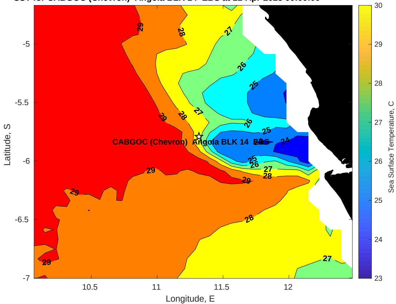
SST for CABGOC (Chevron) Angola BLK 14 EBS at 11-Apr-2025 00:00:00
