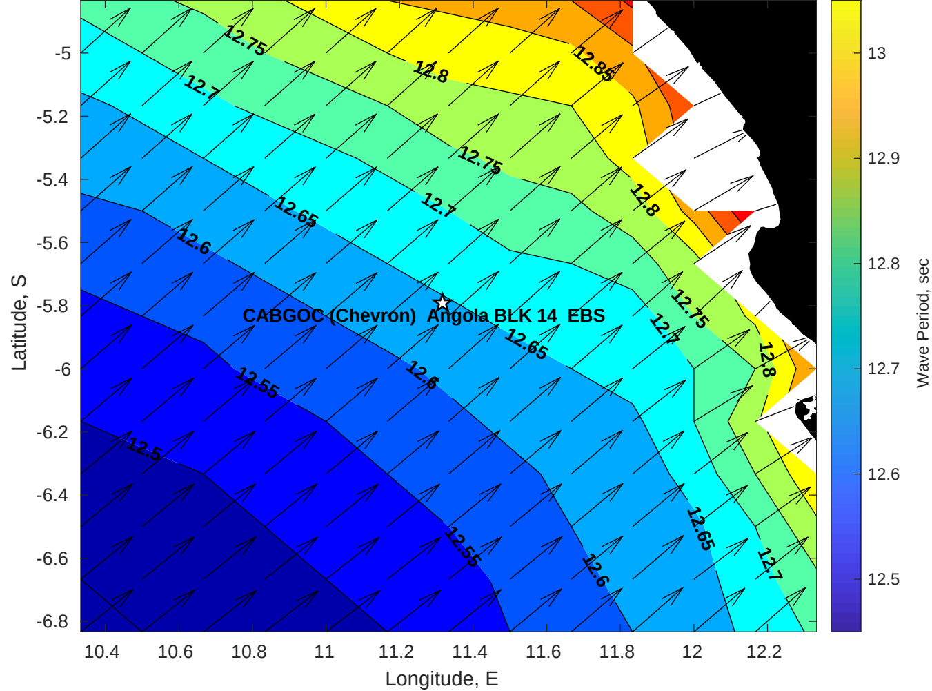
Wave Period (sec) for CABGOC (Chevron) Angola BLK 14 EBS at 12-Apr-2025 09:00:00
