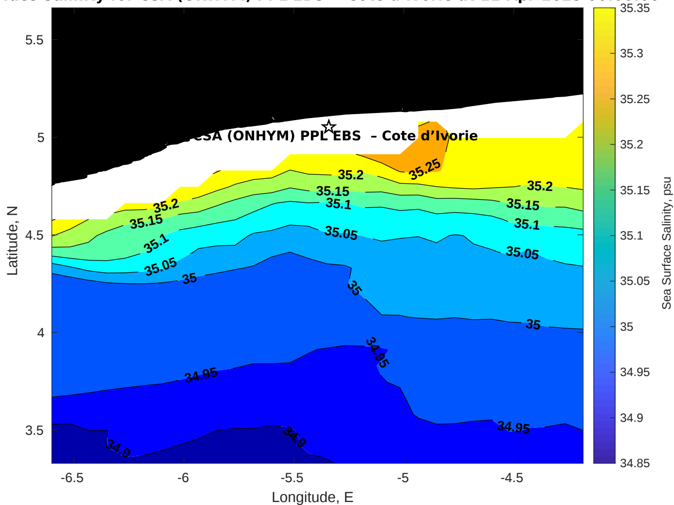
Surface Salinity for CSA (ONHYM) PPL EBS - Cote d'Ivoire at 11-Apr-2025 00:00:00
