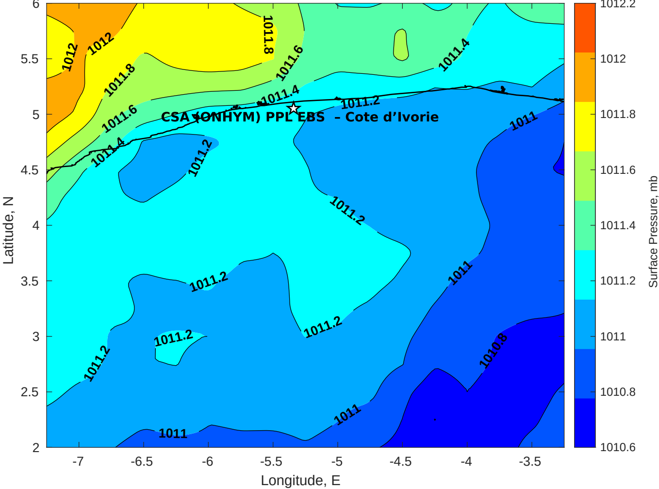
Surface Pressure (mb) for CSA (ONHYM) PPL EBS - Cote d'Ivoire at 13-Apr-2025 00:00:00
