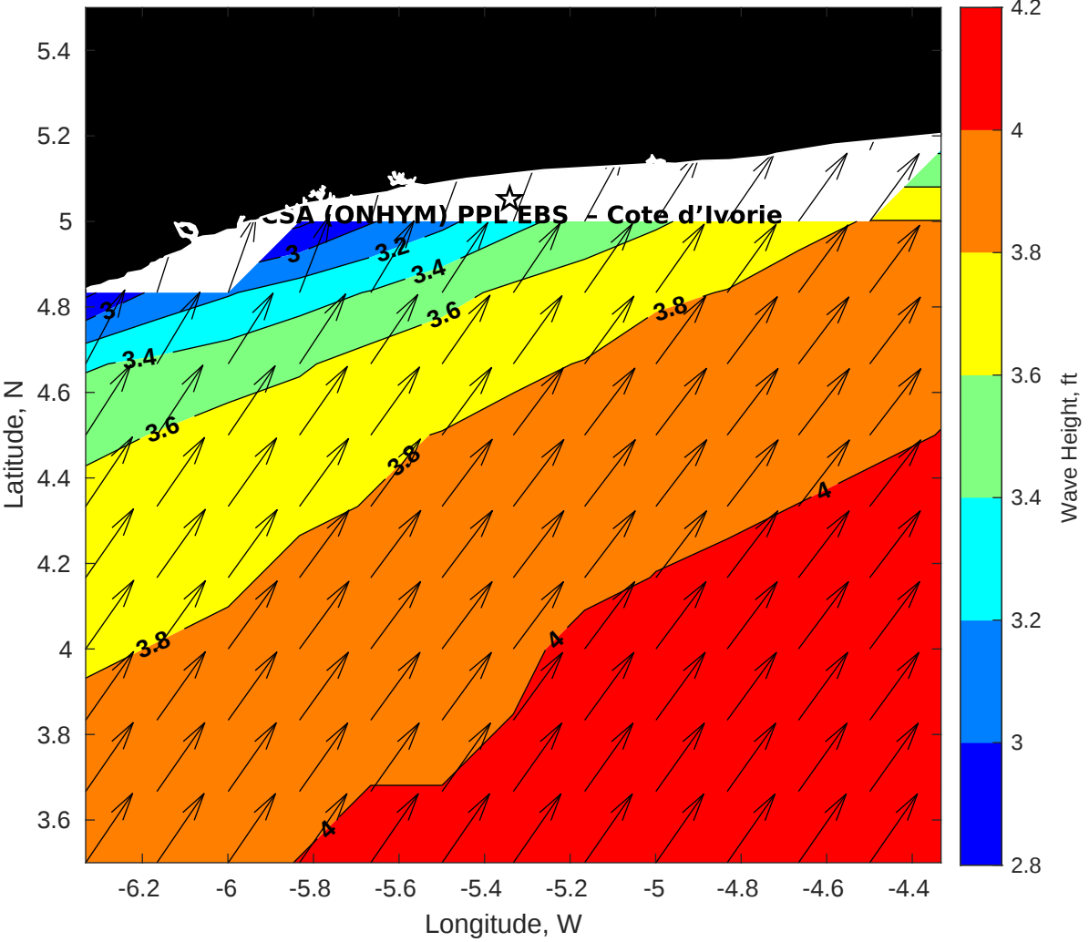
Wave Height (ft) for CSA (ONHYM) PPL EBS - Cote d'Ivoire at 12-Apr-2025 09:00:00
