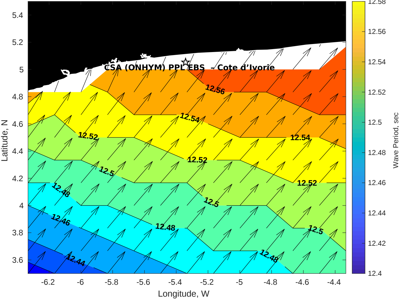
Wave Period (sec) for CSA (ONHYM) PPL EBS - Cote d'Ivoire at 12-Apr-2025 09:00:00
