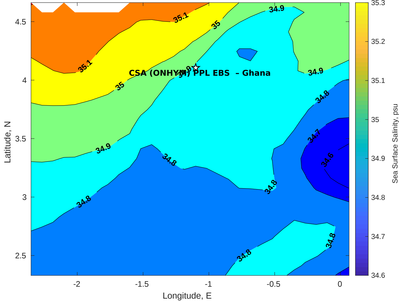
Surface Salinity for CSA (ONHYM) PPL EBS - Ghana at 11-Apr-2025 00:00:00
