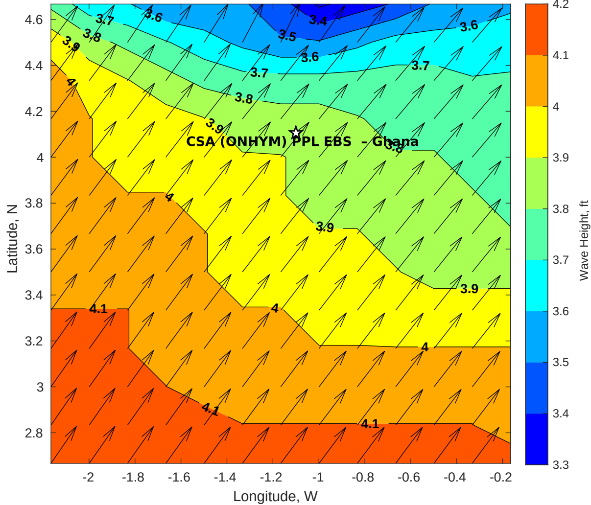
Wave Height (ft) for CSA (ONHYM) PPL EBS - Ghana at 12-Apr-2025 09:00:00
