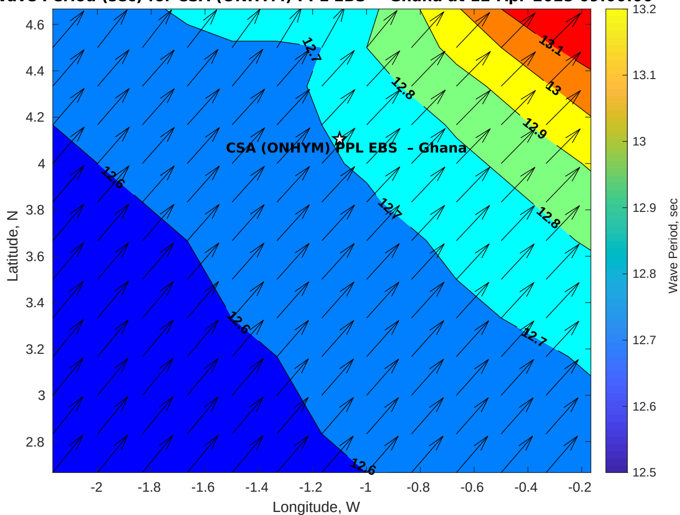
Wave Period (sec) for CSA (ONHYM) PPL EBS - Ghana at 12-Apr-2025 09:00:00
