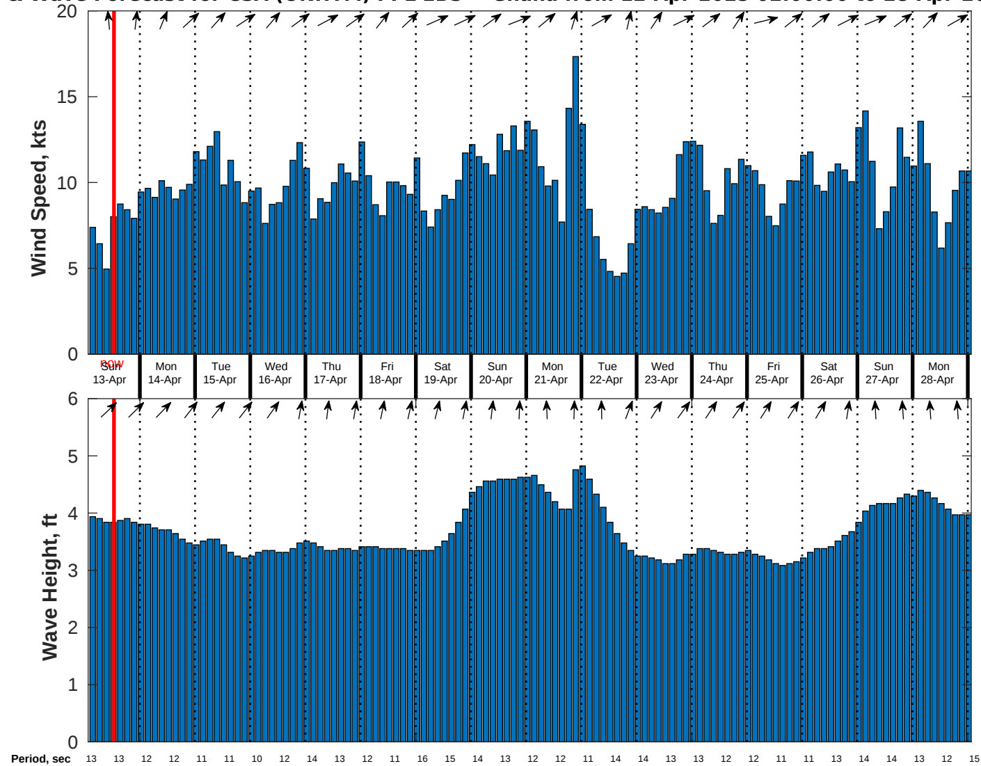
Wind & Wave Forecast for CSA (ONHYM) PPL EBS - Ghana from 12-Apr-2025 02:00:00 to 28-Apr-2025 02:00:00
