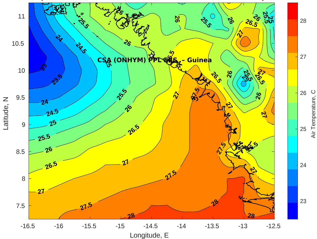
Air Temperature (C) for CSA (ONHYM) PPL EBS - Guinea at 12-Apr-2025
