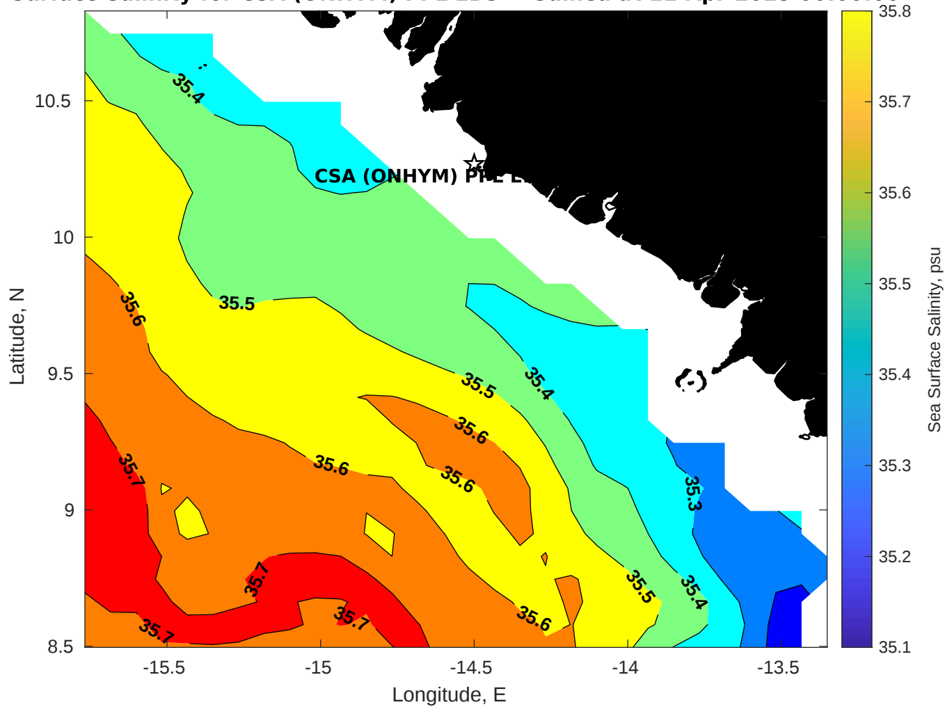
Surface Salinity for CSA (ONHYM) PPL EBS - Guinea at 11-Apr-2025 00:00:00
