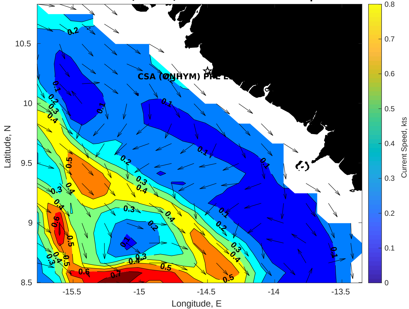
Surface Currents for CSA (ONHYM) PPL EBS - Guinea at 11-Apr-2025 00:00:00
