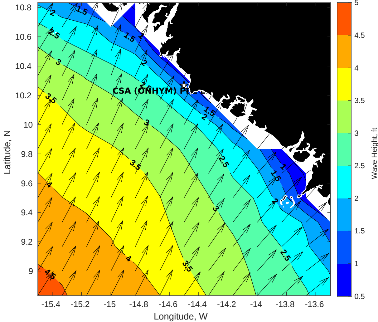
Wave Height (ft) for CSA (ONHYM) PPL EBS - Guinea at 12-Apr-2025 09:00:00
